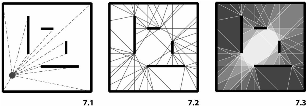
Figure 7. Partitioning of a given shape into convex sub-shapes such that a constant set of end-points and corners is visible from within each sub-shape: Figure 7.1 shows the corners and end-points that have a direct line of sight from a chosen root point; Figure 7.2 shows the sub-division of the given shape into all its constituent sub-shapes; Figure 7.3 shows the graphic representation of centrality relative to visual changes. Distance is counted by the minimum number of sub-shapes that are crossed to go from each sub-shape to all others; lighter shades indicate sub-shapes with high centrality and darker shades those with low centrality (source: the authors).
