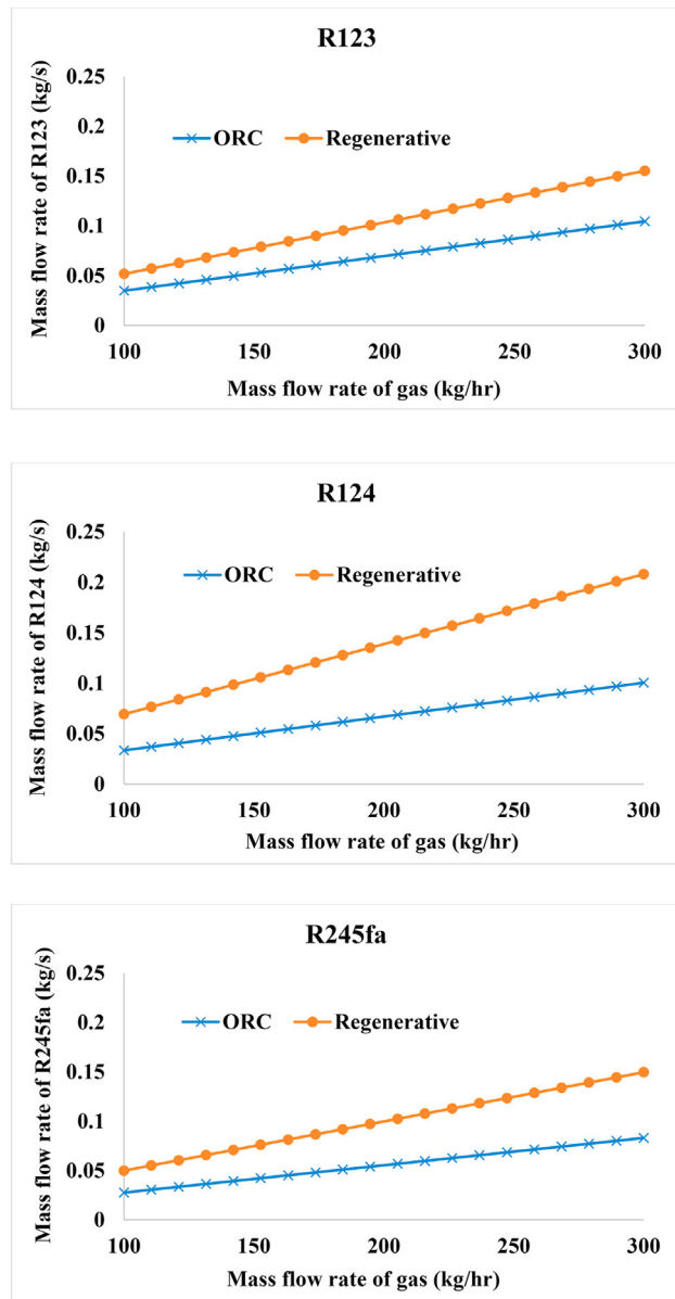
Fig. 12. The relation between mass flow rate of heat source and working fluids in basic and regenerative organic Rankine cycles for (a) R123, (b) R124 and (c) R245fa.
