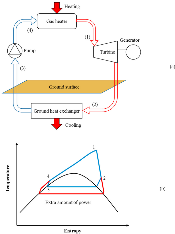
Fig. 2. CO 2 -based transcritical Rankine cycle combined with a ground-cooled condenser; (a) components and (b) temperature-entropy diagram.
