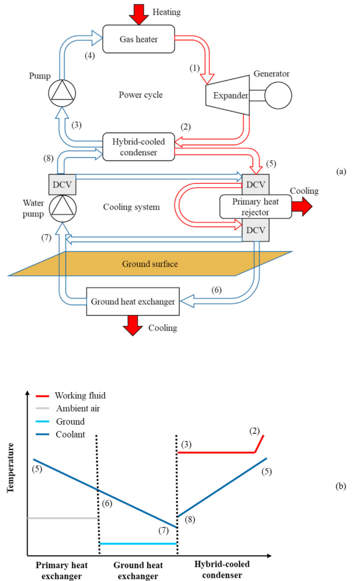
Fig. 3. (a) Schematic diagram of the optimized system and (b) temperature variation in the cooling system; directional control valve (DCV).
