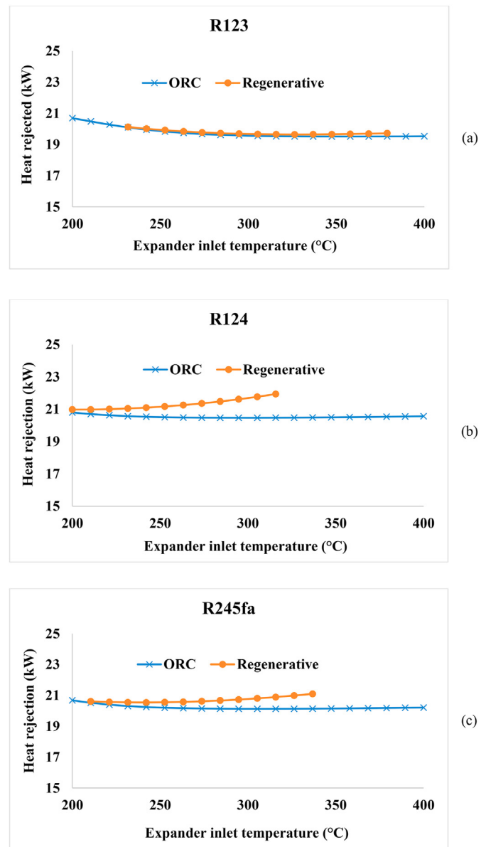
Fig. 13. The influence of regenerator on the heat rejected to the ground for (a) R123, (b) R124 and (c) R245fa.
