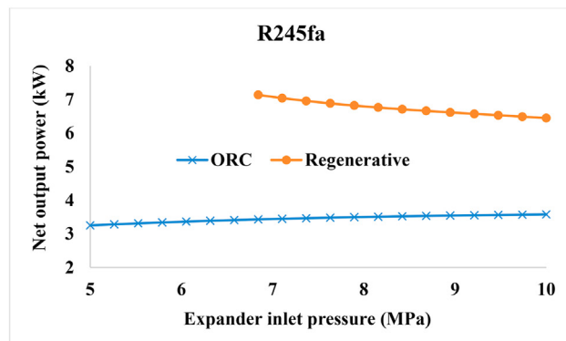
Fig. 10. Effect of expander inlet pressure on the net output power of basic and regenerative organic Rankine cycles for (a) R123, (b) R124 and (c) R245fa.
