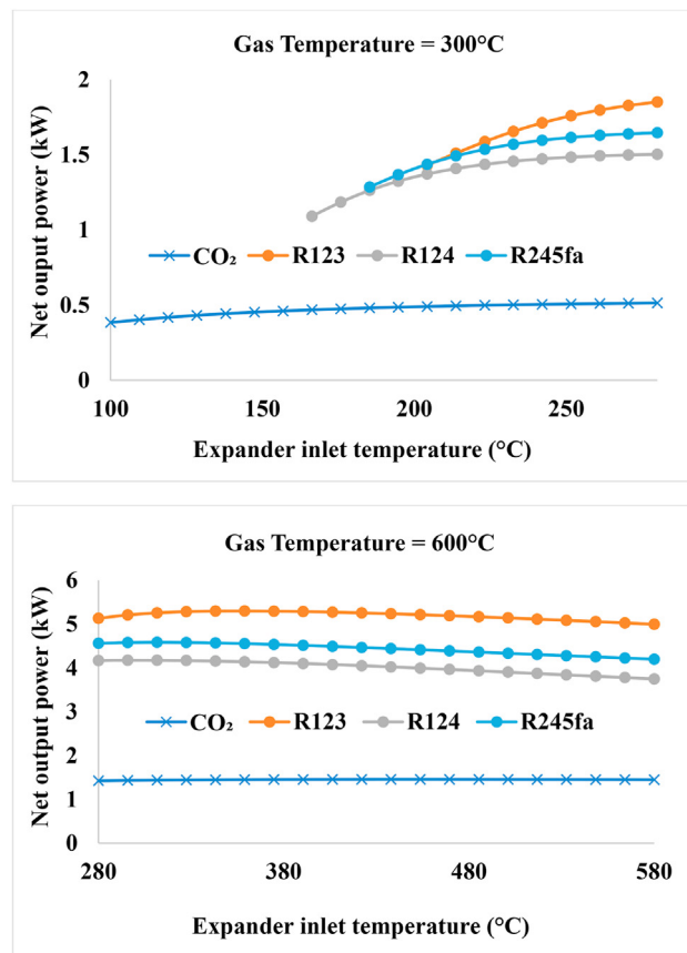
Fig. 4. Effect of expander inlet temperature on the performance of working fluids at gas temperature of (a) 300 °C and (b) 600 °C.
