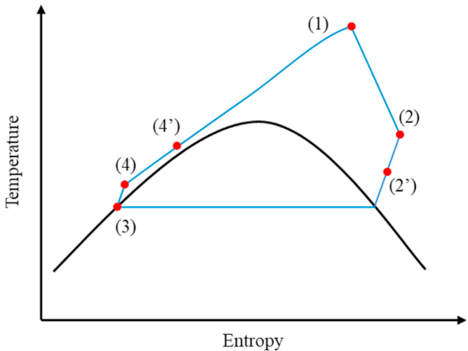
Fig. 8. Temperature-entropy diagram of the regenerative transcritical Rankine cycle.
