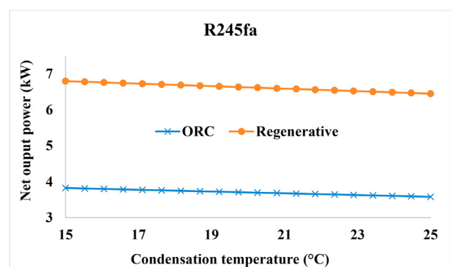
Fig. 11. Effect of condensation temperature on the net output power of basic and regenerative organic Rankine cycles for (a) R123, (b) R124 and (c) R245fa.
