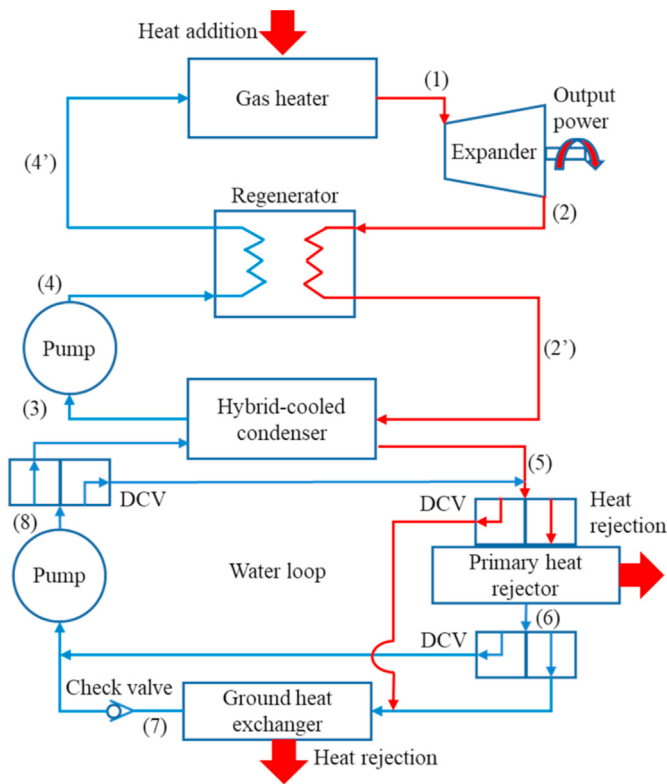
Fig. 7. Schematic diagram of the regenerative cycle.
