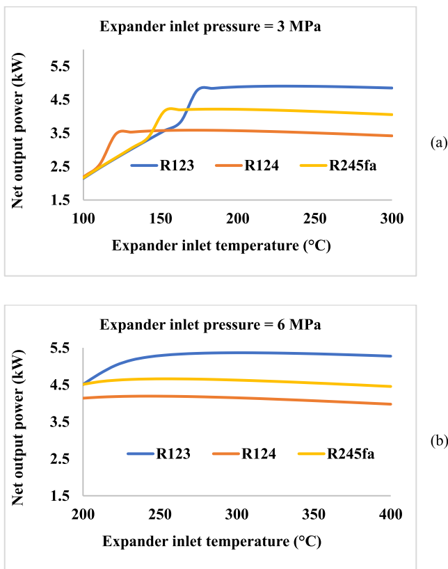
Fig. 6. The variation of net output power as a function of expander inlet temperature at a condensation temperature of 15 °C and expander inlet pressure of (a) 3 MPa and (b) 6 MPa.
