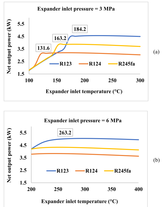
Fig. 5. The best point temperature of investigated working fluids at a condensation temperature of 25 °C and expander inlet pressure of (a) 3 MPa and (b) 6 MPa.
