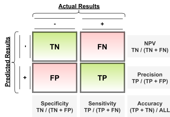
Fig. 8. Summary on the performance metrics from the confusion matrix.
