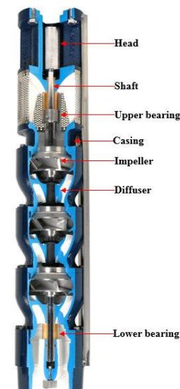
Figure 1: Major components in a multi-stage Electrical Submersible Pump [3]
