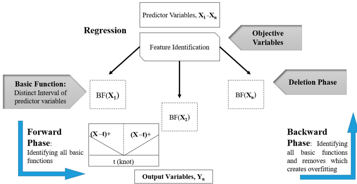
Figure 9. Multivariate adaptive regression splines (MARS).
