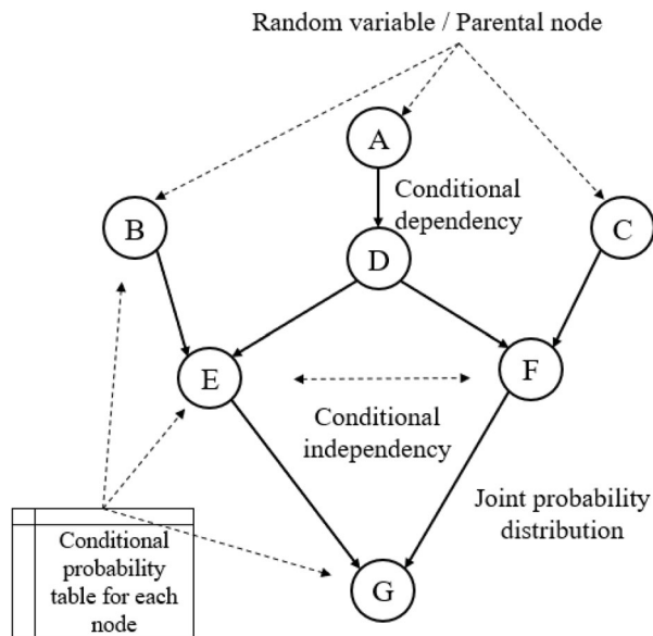
Figure 6. Basic Bayesian network design that satisfies the local Markov property which states that a node conditionally independent of its non-descendants' parent (e.g. E & F). Joint probability (e.g. P(G|F) , product of P(\text{node}|\text{parental node}) ) is calculated using the chain rule of probability.
