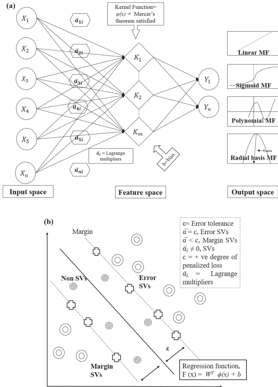
Figure 4. (a) Typical SVM architecture for SSL modeling where \bar{a} = weight and b = bias. Most common transfer functions are linear, polynomial, radial basis, and sigmoidal, K = support vector, m = number of support vectors, \phi(x) = non-linear function. (b). Non-linear SVR vaponik's \epsilon -insensitivity loss function.
