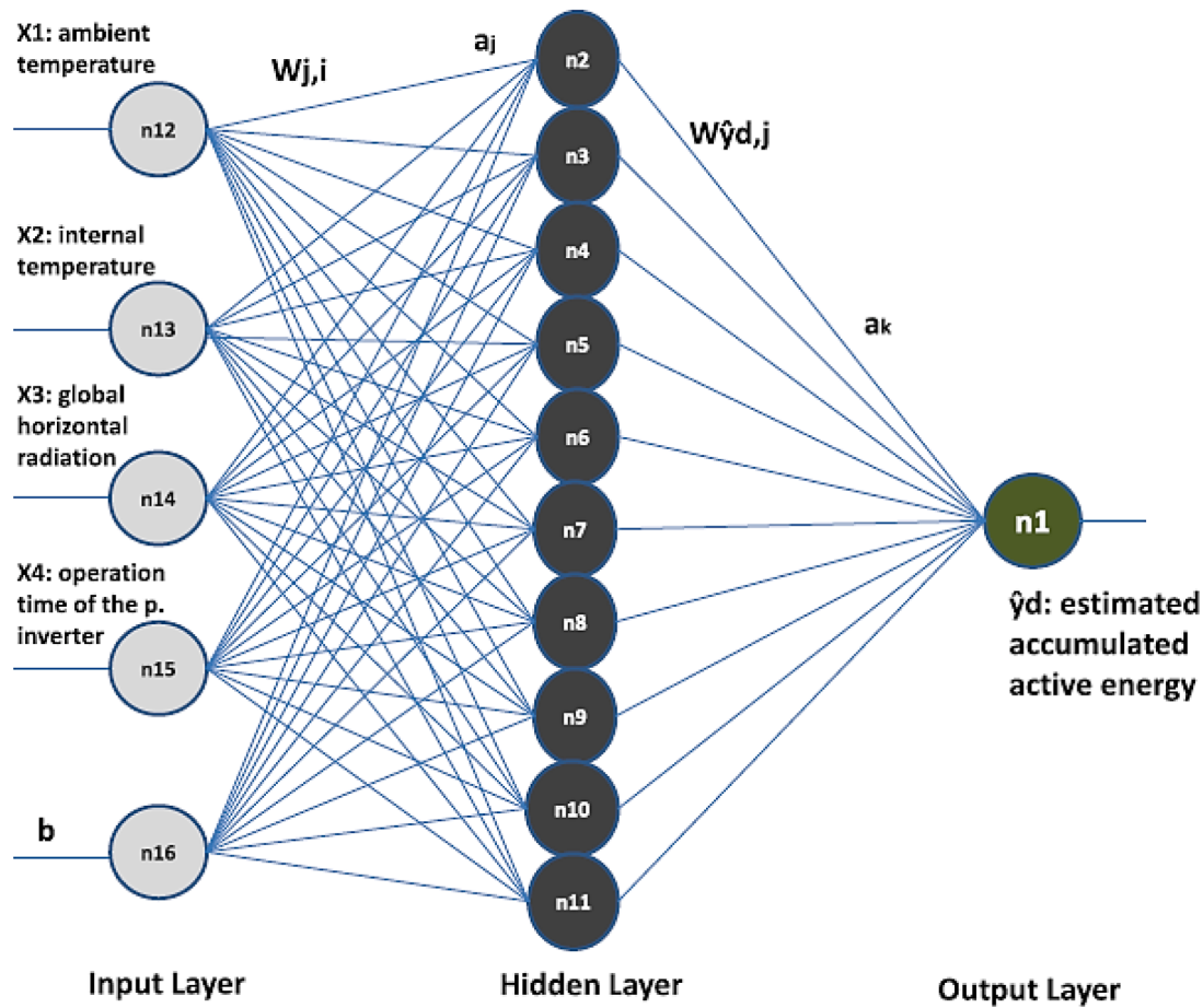
Fig. 9. Multi-layer ANN back propagation [66].
