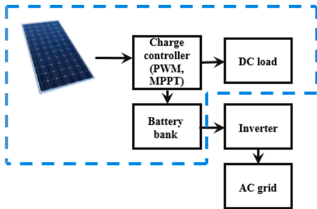
Fig. 10. DC detection zone.
