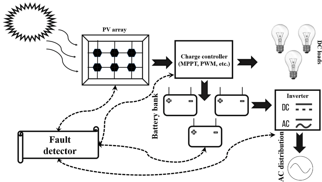
Fig. 1. Fault detector allocation in an off-grid PV system.
