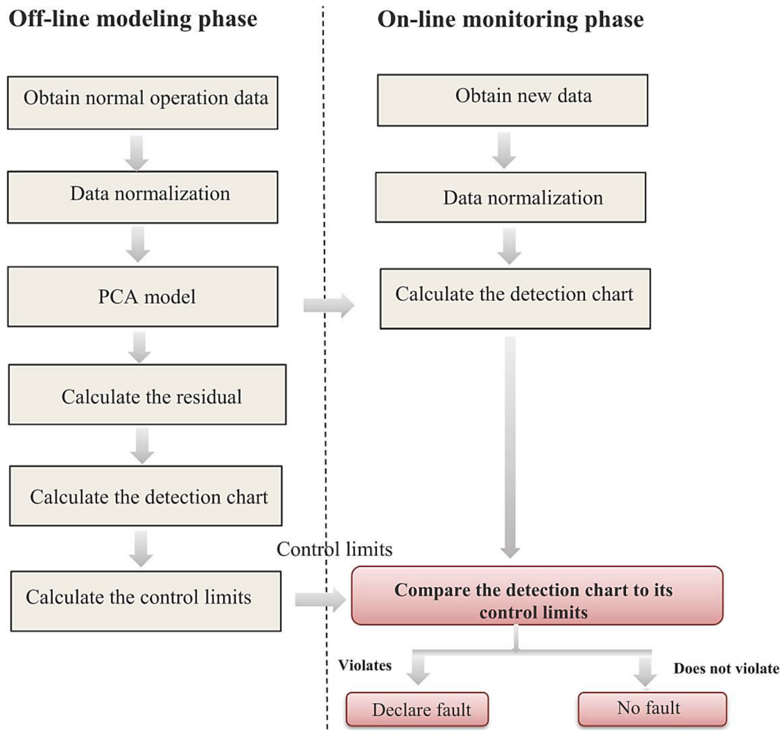
Fig. 12. General diagram of detector scheme [163].
