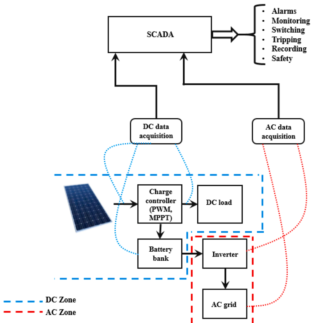
Fig. 19. The suggested AC-DC fault detection general overview.
