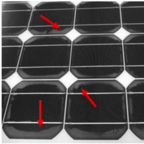
Fig. 5. Delamination of the PV module's front encapsulation [51].
