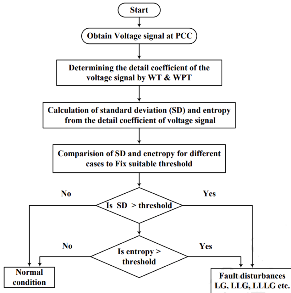
Fig. 13. MWPT flowchart [167].
