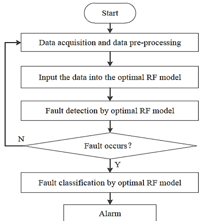
Fig. 14. The RF flowchart [241].
