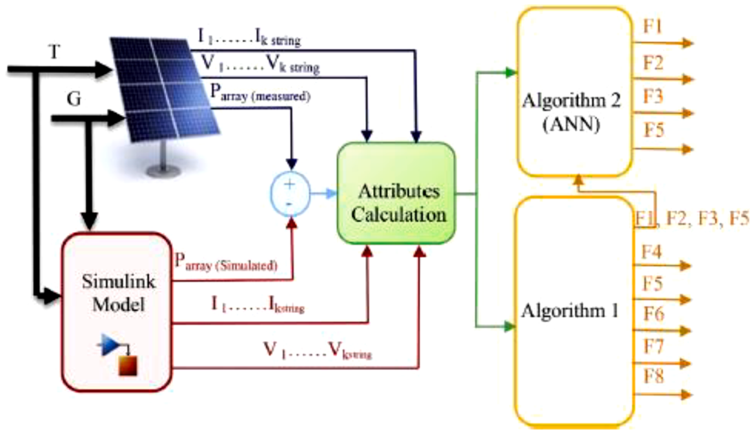
Fig. 16. Two-algorithm ANN proposed fault classifier [60].
