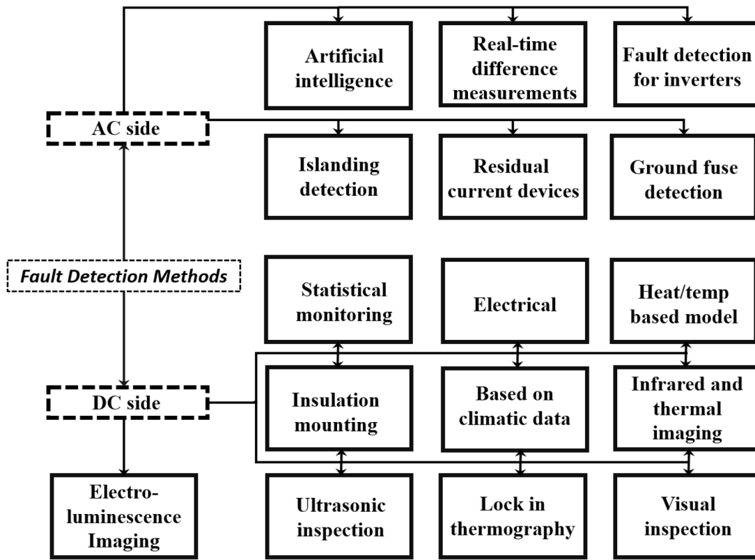
Fig. 6. Complete PV fault detection methods at AC/DC sides of the PV system.
