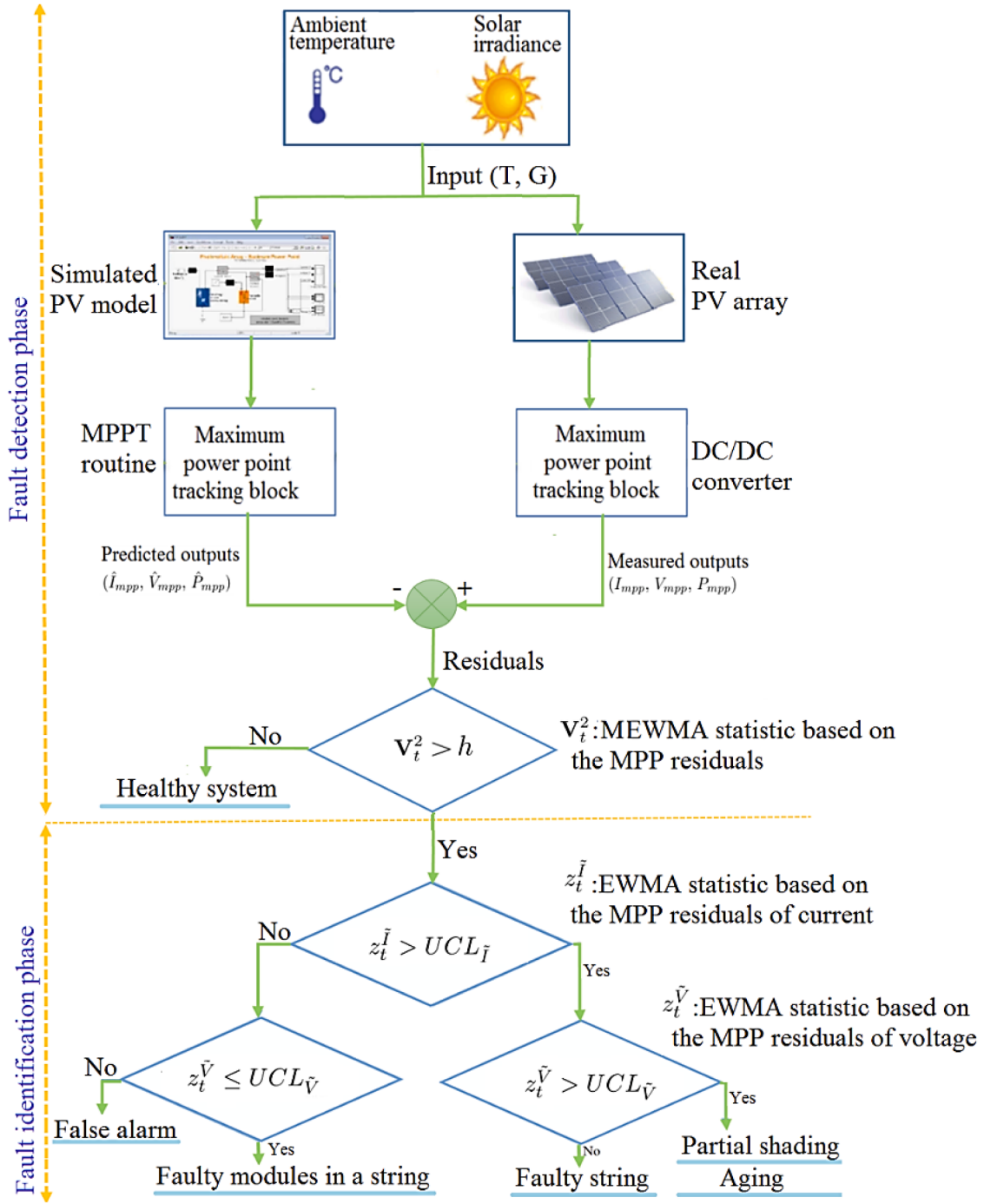
Fig. 11. MEWMA flowchart [169].
