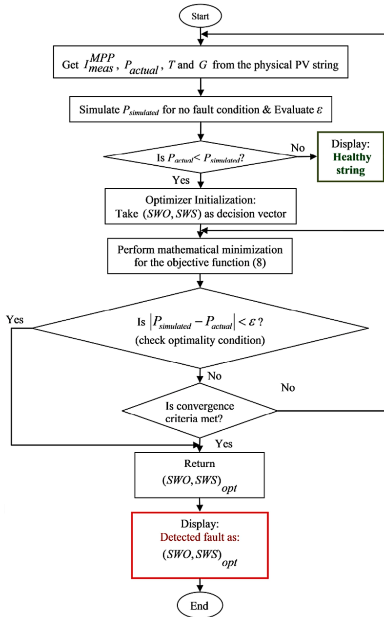
Fig. 17. Solution flowchart [61].
