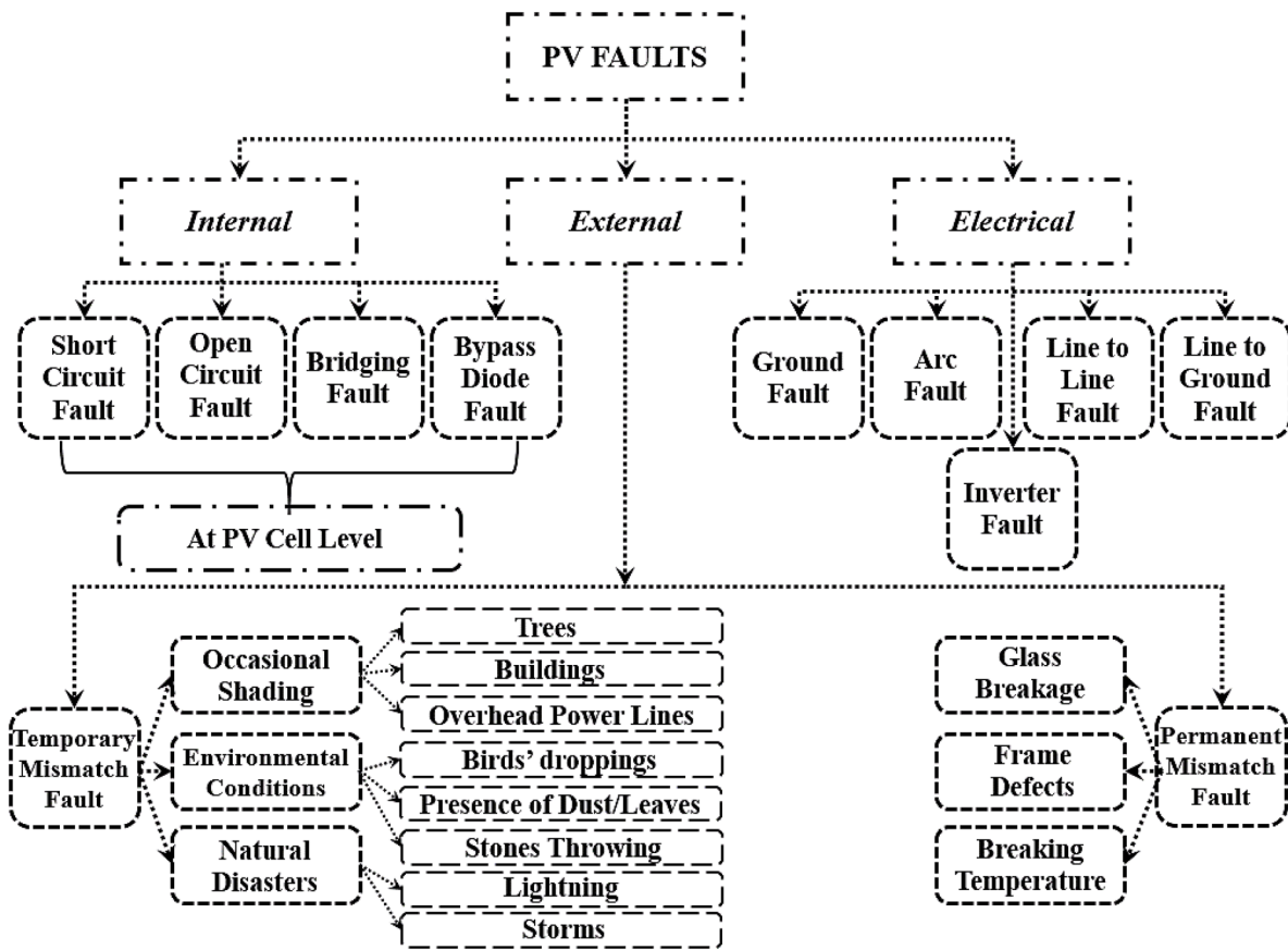
Fig. 4. Summarizing block diagram representation of PV fault types and characterization.
