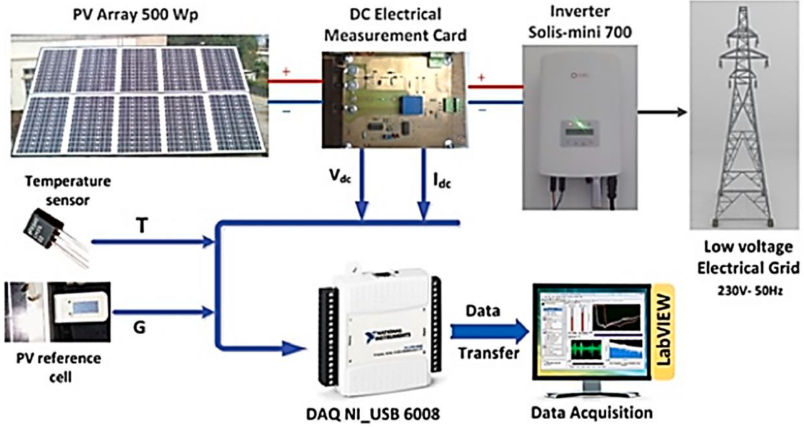
Fig. 8. Synoptic scheme for GCPVS [56].
