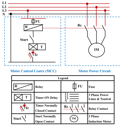
Fig. 1. Schematic of an example MCC.
