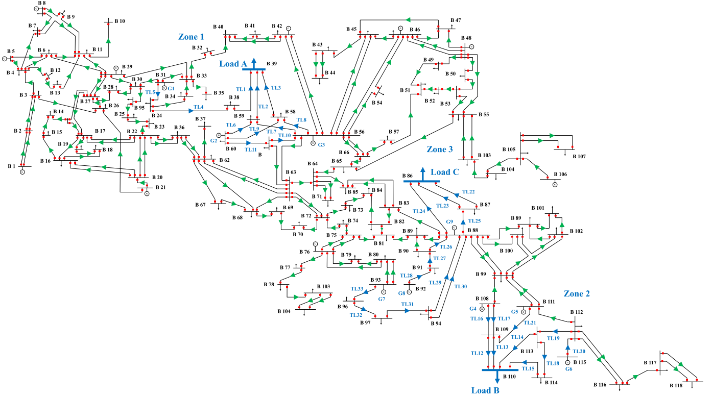
Fig. 4. IEEE 118-bus electrical power grid system.
