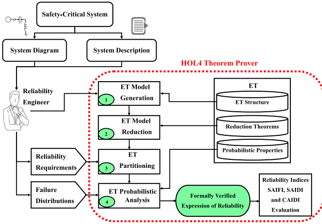
Fig. 3. Methodology for formal probabilistic ET analysis.
