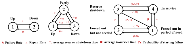
Fig. 5. Multistate models for reliability studies.
