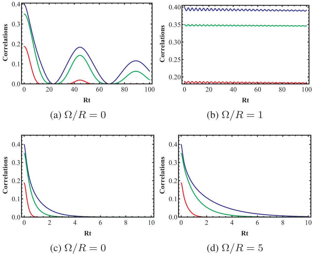
Fig. 4. Quantum and classical correlations as a function of the dimensionless time Rt for the initial entangled mixed state \rho = 1/3[|(1-a)|++\rangle\langle++| + 2|\Psi\rangle\langle\Psi| + a|--\rangle\langle--|] in different driving strengths \Omega/R of the external classical field with a = 1/2 . Panels (a) and (b) exhibit the strong-coupling regime ( \lambda = 0.01R ), where panels (c) and (d) exhibit the weak-coupling regime ( \lambda = 10R ). The blue solid line is for the quantum discord, Red solid line is for the entanglement of formation, and green solid line is for the classical correlation. (For interpretation of the references to colour in this figure legend, the reader is referred to the web version of this article.)
