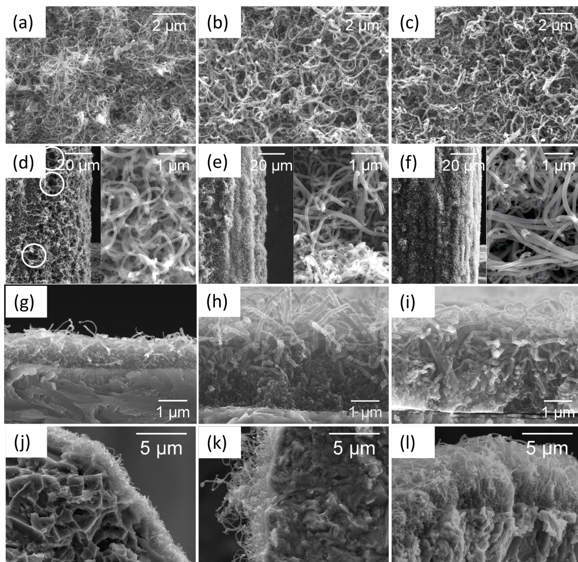
Figure 2. SEM micrographs of NCNTs on: a–c) Ti foil, and d–f) Ti mesh showing the effect of t_1 . a, d) t_1 = 60 s, b, e) t_1 = 90 s, and c, f) t_1 = 120 s, t_2 = 10 s. The growth time ( t_2 ) is 90 min, the substrate temperature is 600 °C. SEM micrographs of NCNTs on: g–i) Ti foil, and j–l) Ti mesh showing the effect of t_2 . g, j) t_2 = 60 min, h, k) t_2 = 90 min, and i, l) t_2 = 120 min (Fe electrodeposition in all cases with t_1 = 90 s and t_2 = 10 s). Circles in Figure 2d indicate voids in the nanotube layer.
