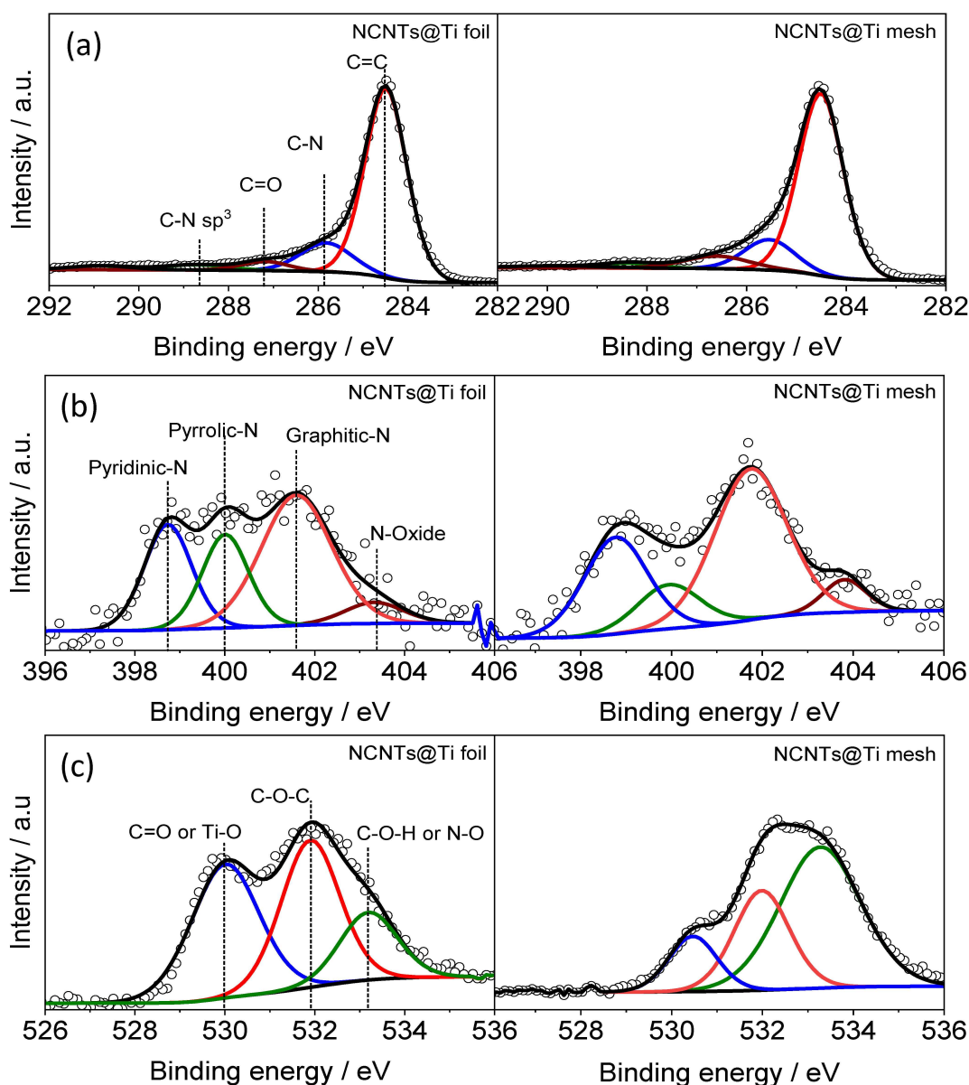
Figure 5. XPS high-resolution spectra of NCNTs on Ti foil and Ti mesh. a) C 1 s, b) N 1 s, and c) O 1 s t_1 = 90 s, t_2 = 10 s, t_3 = 90 min, T_3 = 600 °C.
