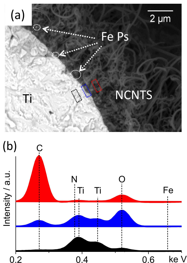
Figure 3. a) SEM-BSE micrographs of as-grown NCNTs on Ti mesh. b) EDX analysis along area marked in black, blue, and red in Figure 3a. t_1 = 90 s, t_2 = 10 s, t_G = 90 min, T_S = 600^\circ\text{C} .
