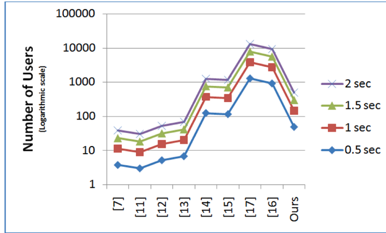
Fig. 6. Number of users authenticated.
