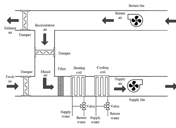
Figure 6. Schematic diagram of an AHU (Y. Yan et al., 2020)
