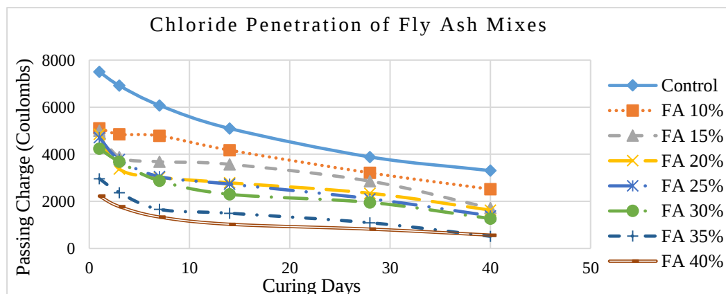
Figure 2. Chloride Penetration of Fly Ash Mixes
