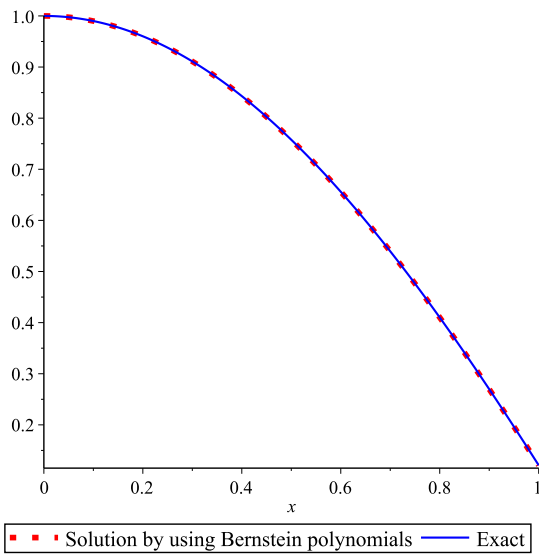
Fig. 3. Approximation solution for example 3 using Bernstein polynomials with exact solution.
