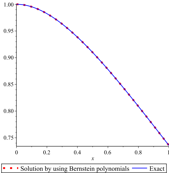
Fig. 2. Approximation solution for example 2 using Bernstein polynomials with exact solution.
