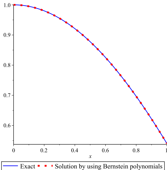
Fig. 1. Approximation solution for example 1 using Bernstein polynomials with exact solution.
