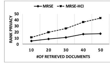
Fig. 13. Rank privacy.
