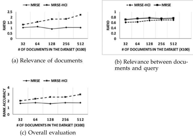
Fig. 12. Search precision.
