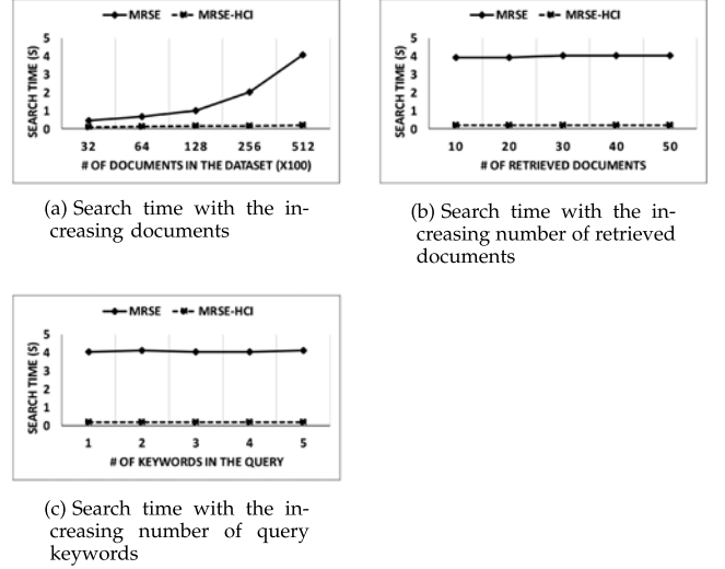
Fig. 11. Search efficiency.
