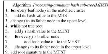
Fig. 9. Algorithm processing-minimum hash sub-tree.
