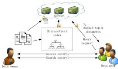
Fig. 1. Architecture of ciphertext search.
