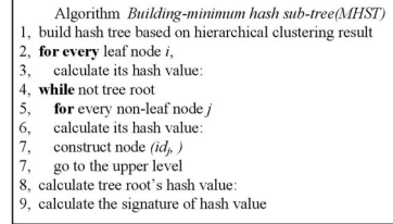
Fig. 8. Algorithm building-minimum hash sub-tree.
