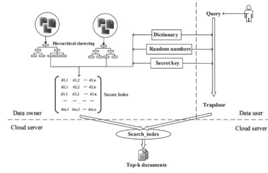
Fig. 2. MRSE-HCI architecture.
