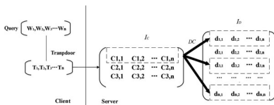
Fig. 7. Retrieval process.
