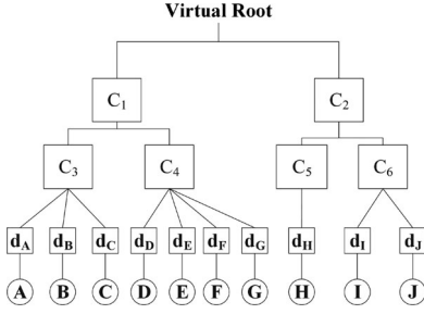
Fig. 10. Authentication for hierarchical clustering index.
