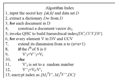
Fig. 3. Algorithm index.
