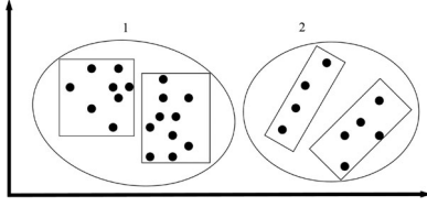
Fig. 6. Clustering process.
