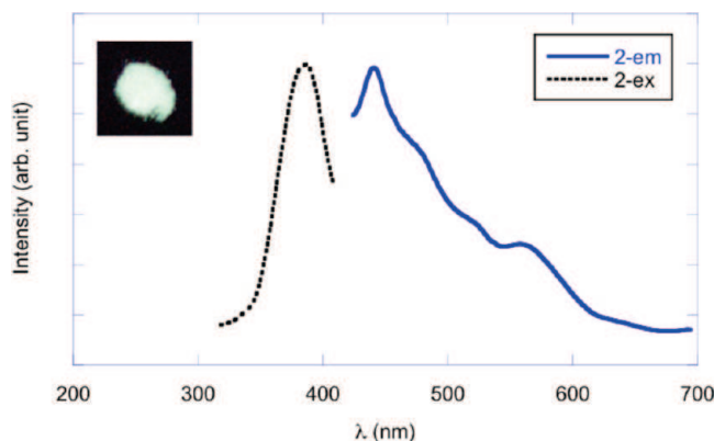
Figure 10. Excitation (ex; dotted line) and emission (em; solid line) spectra of compound 2 . Inset is an optical image of the “white” luminescent compound 2 .
