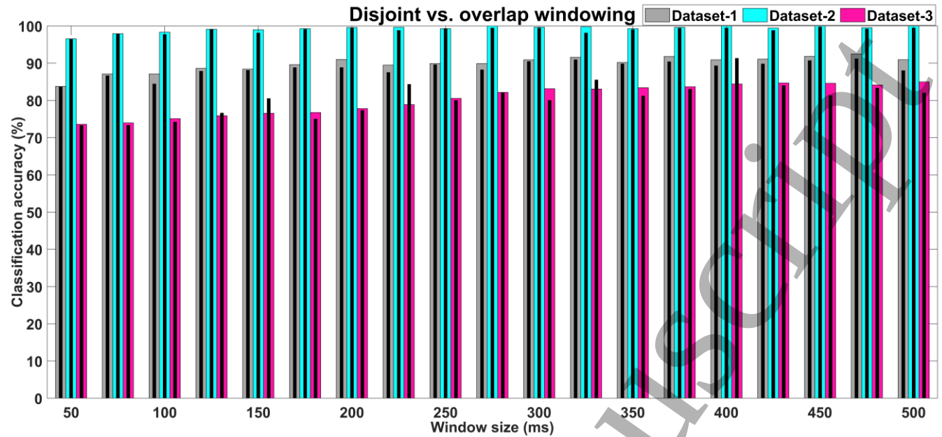
Figure 9. Comparison of MCA for overlap and disjoint windowing techniques for all datasets on all 19 different window sizes. It can be observed that on each individual window size, the overlap windowing technique outperforms disjoint windowing technique in terms of MCA.
