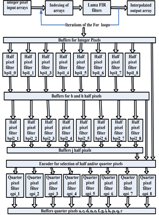
Figure 2. HLS implementation of H.264/AVC Luma Sub-pixel.
