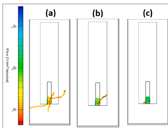
Fig. 11. Side view of \beta^- particle fluence of GOAg:I-131 sediment at (a) 1.0 mg/mL, (b) 3.0 mg/mL, and (c) 5.0 mg/mL in the dose calibrator.
