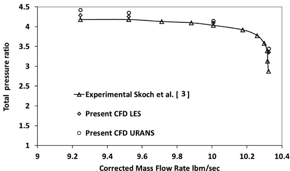
Fig. 4. Pressure ratio of the compressor stage for the CFD results obtained by the URANS and LES models, and previously reported experimental results [3].
