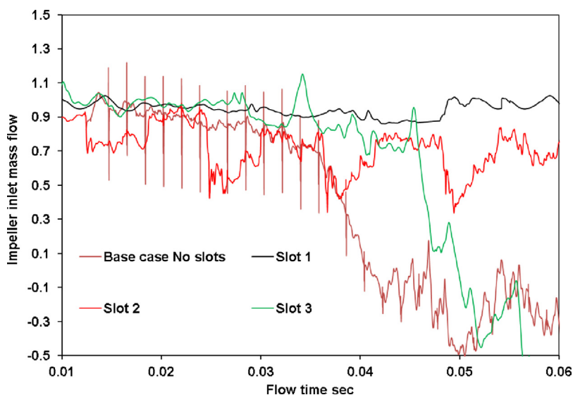
Fig. 9. Dimensionless impeller inlet mass flow caused by the operating mass flow.
