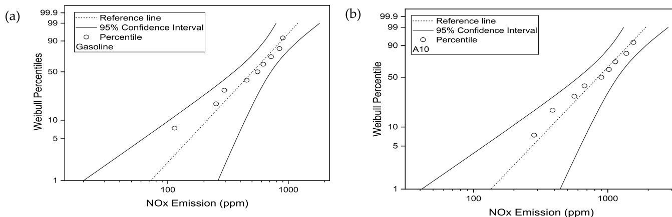
Figure 13. (a) NO x emission Weibull probability against 95% CI for gasoline; (b) NO x emission Weibull probability against 95% CI for A10.
