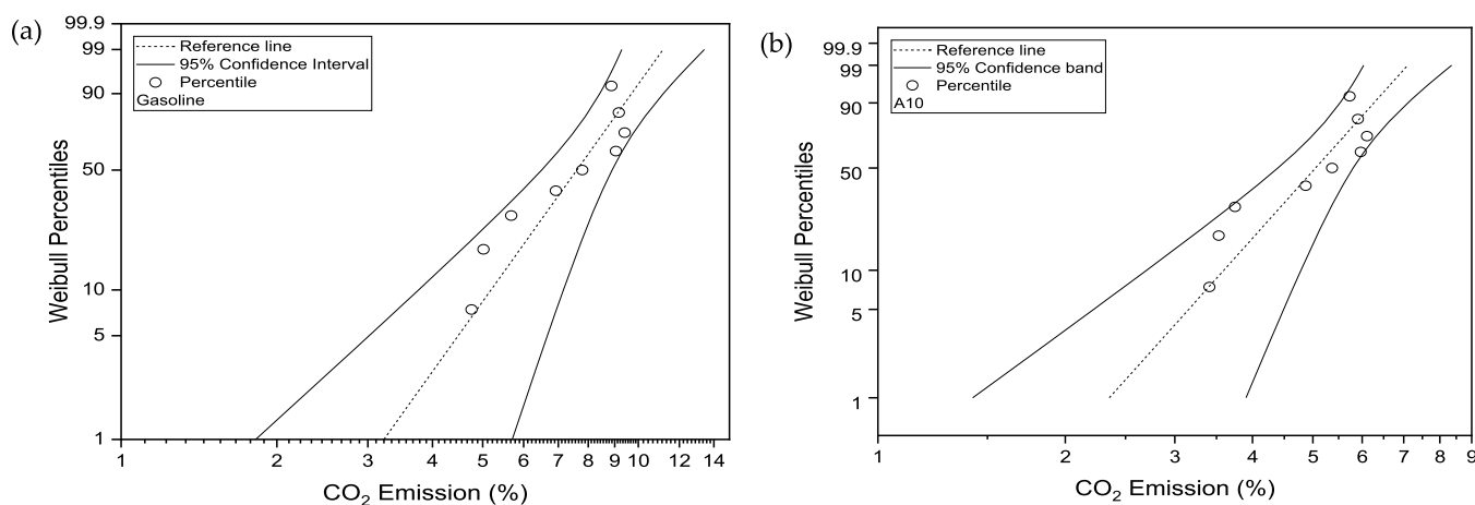
Figure 9. (a) CO 2 emission Weibull probability against 95% CI for gasoline; (b) CO 2 emission Weibull probability against 95% CI for A10.
