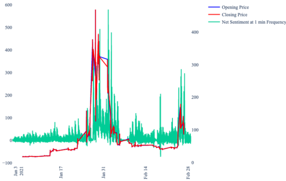
(b) 1-minute net sentiment and GME returns
