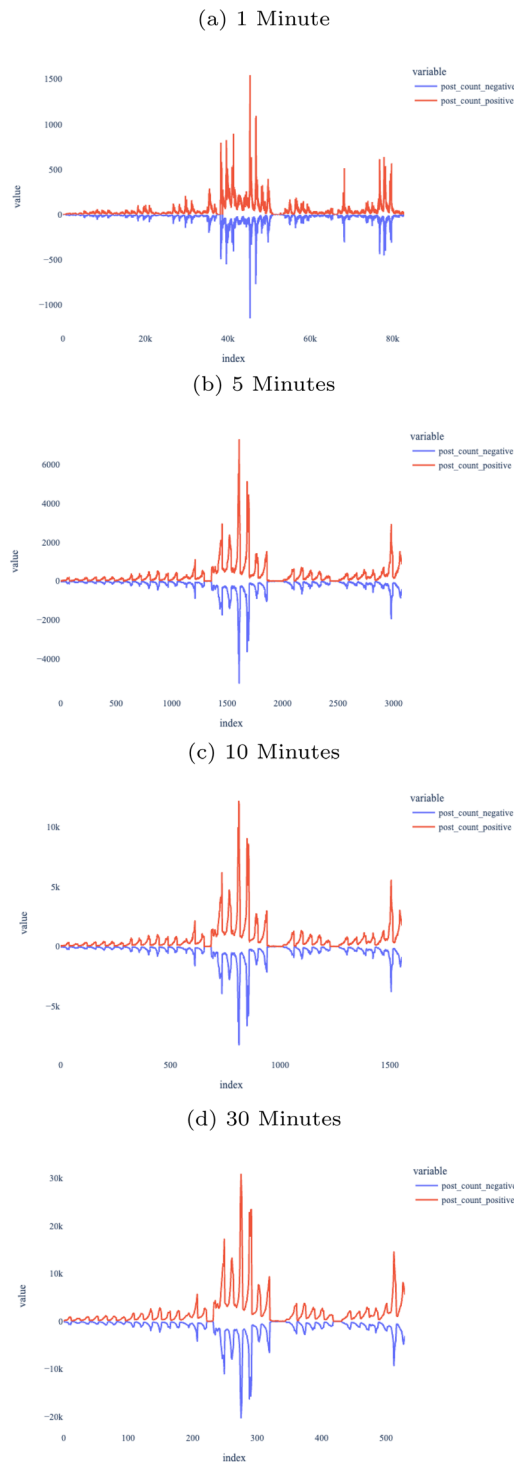
FIGURE 3 Positive and Negative Sentiments at different frequencies
