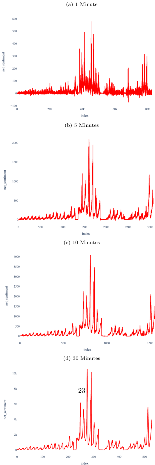
FIGURE 4 Net Sentiments at different frequencies
