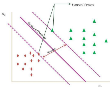
Figure 2: SVM Based Classification
