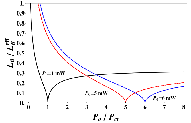
Fig. 1. (Color online) Evolution of the inverse effective beat length versus P_{cr} . Different P_0 are considered.
