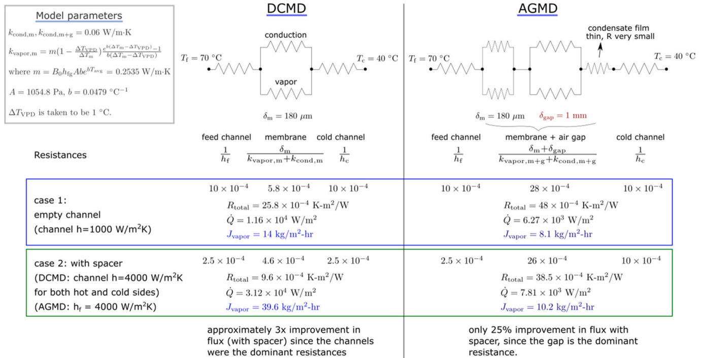
Fig. 6. Comparison of local water flux in DCMD and AGMD based on a simple resistance network model of both processes adapted from [59,60]. Since the channel constitutes the major thermal resistance in DCMD, increasing the channel heat transfer coefficients by four-fold results in about 2.8 times higher flux. On the other hand, in AGMD, the gap constitutes the major thermal resistance. Therefore, increasing the heat transfer coefficient of the feed flow channel by four-fold, as in this study, results in an overall flux improvement of about 25% only.
