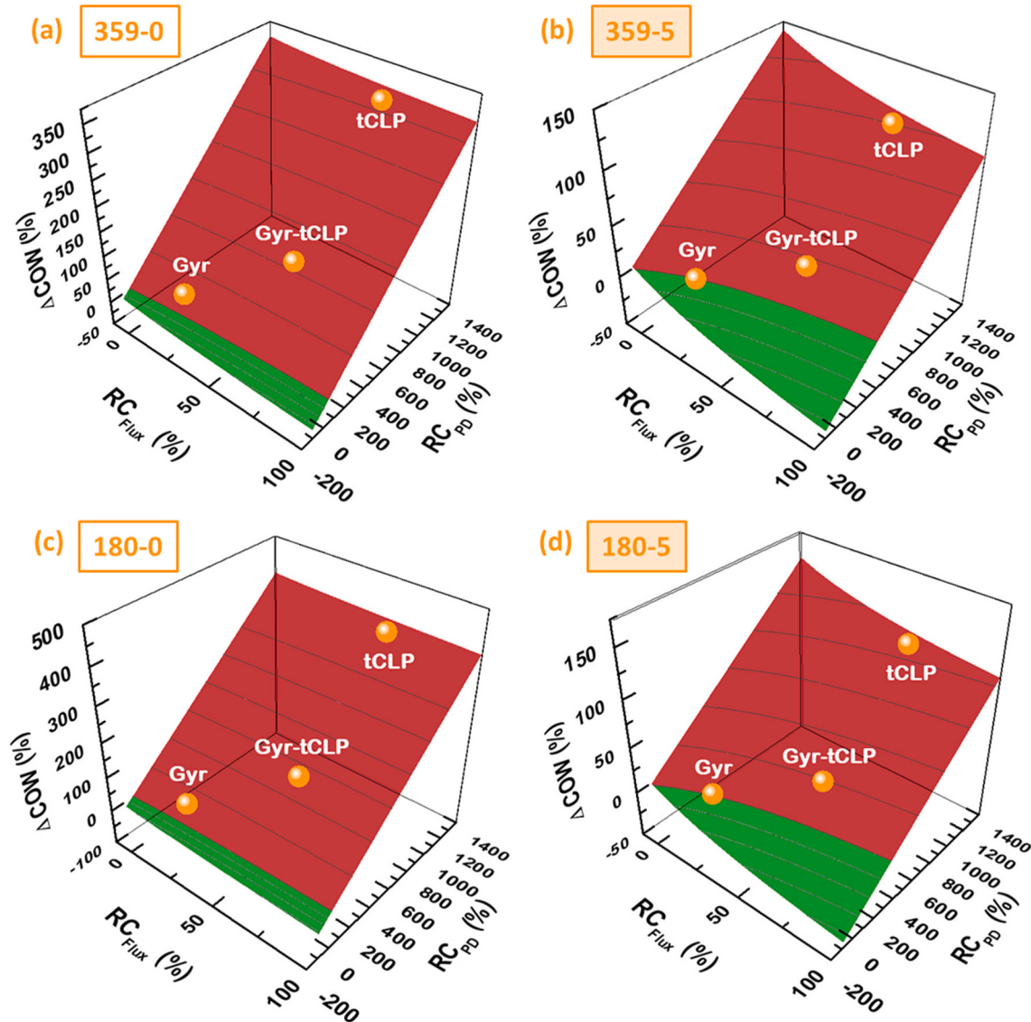
Fig. 9. Cost analysis for a large-scale ( 1000 \text{ m}^3/\text{day} ) DCMD. Trends of the relative COW change when using TPMS spacers instead of CS are plotted for two different values of MD reference CAPEX (current: \$359/\text{m}^2 and prospective: \$180/\text{m}^2 ) and two scenarios: free (waste) heat (left plots) and additional heat costs of \$5/\text{m}^3 (right plots). The green region of the curve is that of a favorable negative variation, or a relative decrease in COW. The red region shows a positive variation, or a relative increase in COW. Results for the TPMS spacers considered in this work are also shown on the curve.
