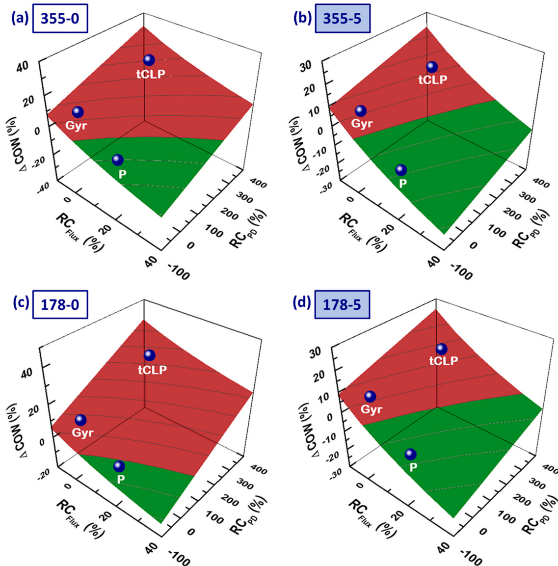
Fig. 8. Cost analysis for a small-scale ( 10 \text{ m}^3/\text{day} ) AGMD. Trends of the relative COW change when using TPMS spacers instead of CS are plotted for two different values of MD reference CAPEX (current: \$355/\text{m}^2 and prospective: \$178/\text{m}^2 ) and two scenarios: free (waste) heat (left plots) and additional heat costs of \$5/\text{m}^3 (right plots). The green region of the curve is that of a favorable negative variation, or a relative decrease in COW. The red region shows a positive variation, or a relative increase in COW. Results for the TPMS spacers considered in this work are also shown on the curve.
