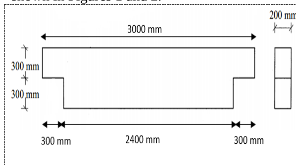
Figure 1. Dapped end beam configuration.
