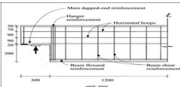
Figure 2. Reinforcement layout of modelled beam.
