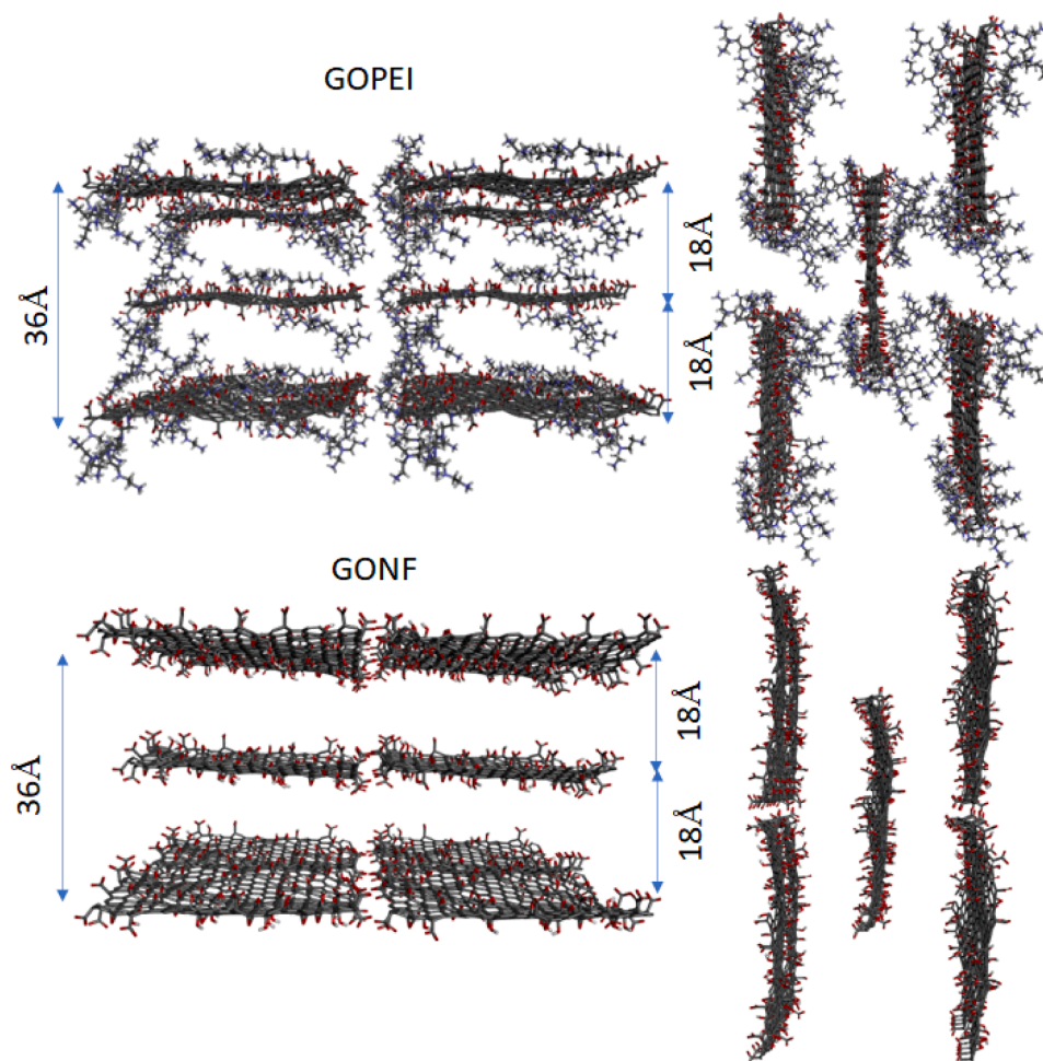
Fig. 2. The 4(top layer)–2(middle layer)–4(bottom layer) configuration of the constructed membranes. The separation between the basal GO planes was constructed to be initially the same for both kinds of membranes. Water molecules used for the hydration of the membranes are omitted for clarity.
