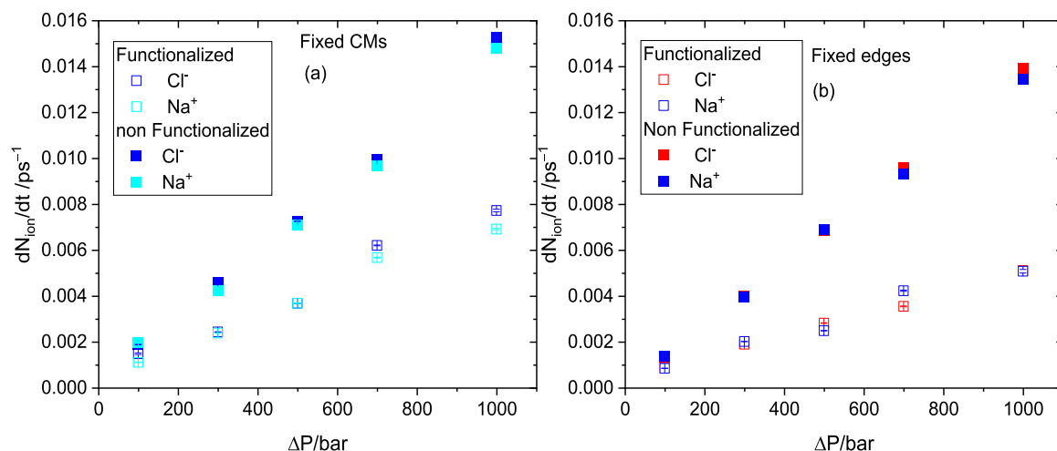
Fig. 10. The rates (number of ions per unit time) of ion-crossing to the permeate as a function of the applied pressure difference for (a) the fixed CMs and (b) the fixed edges models. Error bars are comparable to the size of the symbols.
