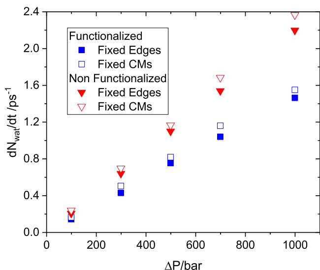
Fig. 6. Water fluxes as a function of the applied pressure difference. Error bars are comparable in size or smaller to the size of the symbols.
