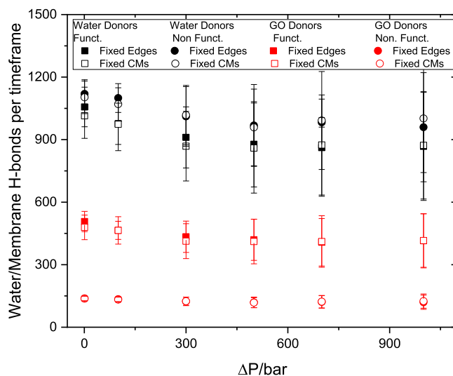
Fig. 8. Hydrogen bonds formed between water molecules and GO flakes of the membrane as a function of the applied pressure gradient. Error bars denote standard deviations.
