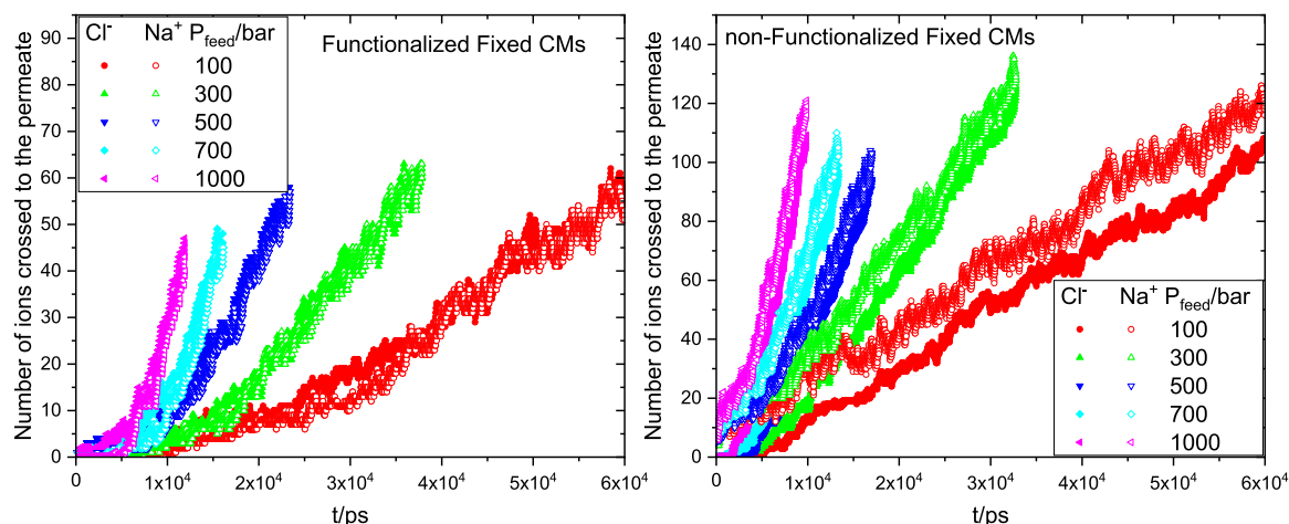
Fig. 9. The number of salt ions present in the permeate as a function of time for the fixed CMs models.
