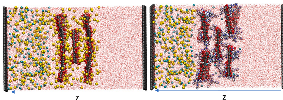
Fig. 3. Initial setups of the GONF-based (left) and the GOPEI-based (right) simulated systems. Carbon atoms are shown in gray, oxygen atoms in red, hydrogen atoms in white, nitrogen atoms in blue, sodium atoms in yellow and chlorine atoms in dark cyan. Water atoms appear as red and white dots. The simulation box boundaries including the extra vacuum space is not shown. Arrows denote the direction of the positive z coordinate.
