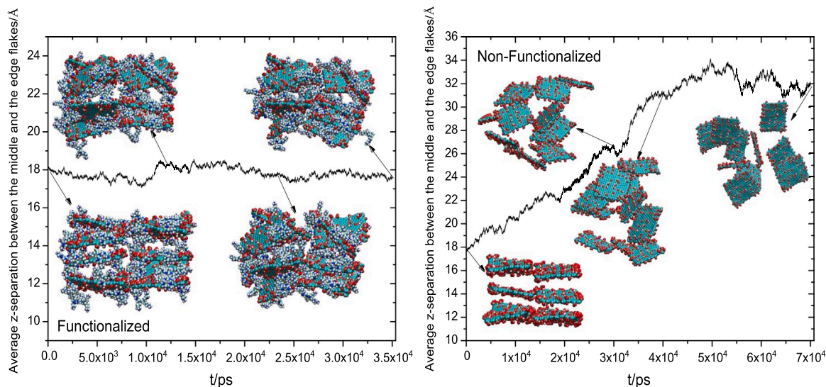
Fig. 13. Average z-separation between the flakes of the middle and the outer layers as a function of the time elapsed during an unconstrained simulation. Snapshots of the membrane are shown at different time instants, denoted by the arrows.
