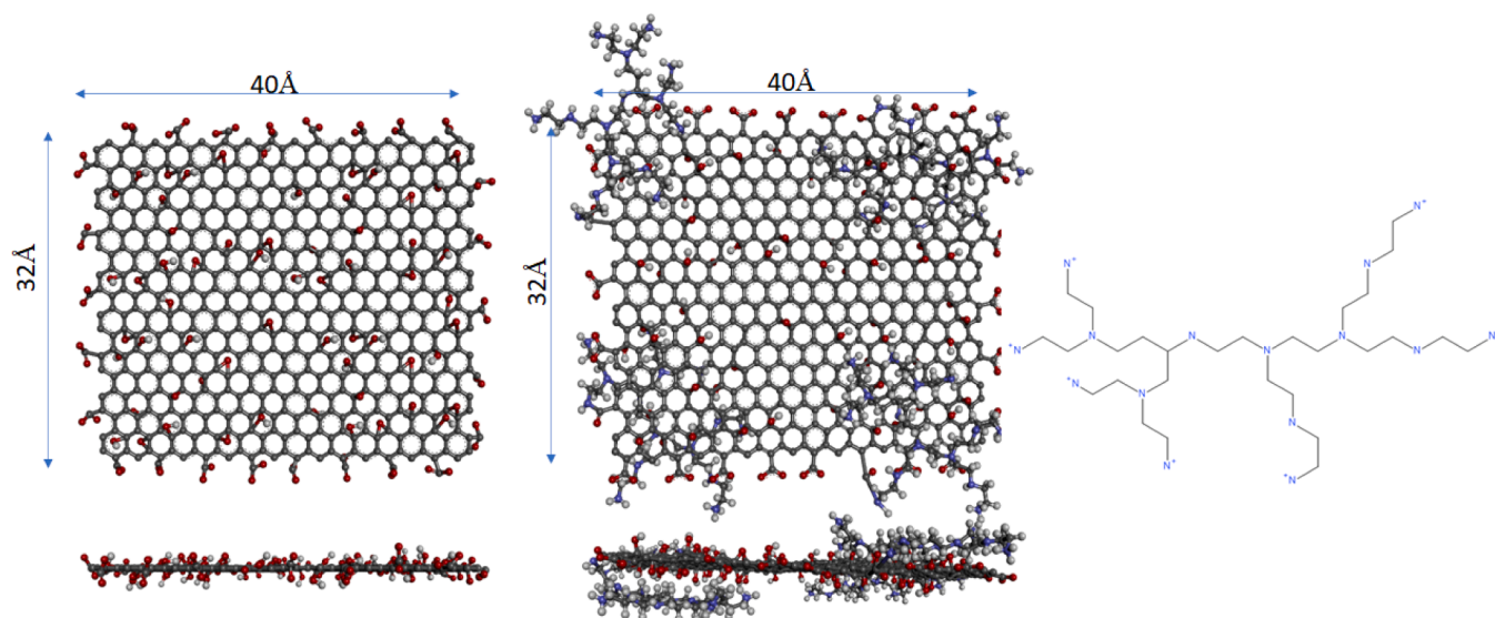
Fig. 1. (Left) A non-functionalized, C 554 H 36 O 112 , and (middle) a branched PEI-functionalized, C 666 H 348 N 60 O 108 , GO flake in frontal and lateral view. Carbon atoms are depicted in dark gray, oxygen atoms in red, hydrogen atoms in white and nitrogen atoms in blue. A schematic of the branched PEI used for the functionalization of the GO nanosheets is shown at the rightmost part of the figure.
