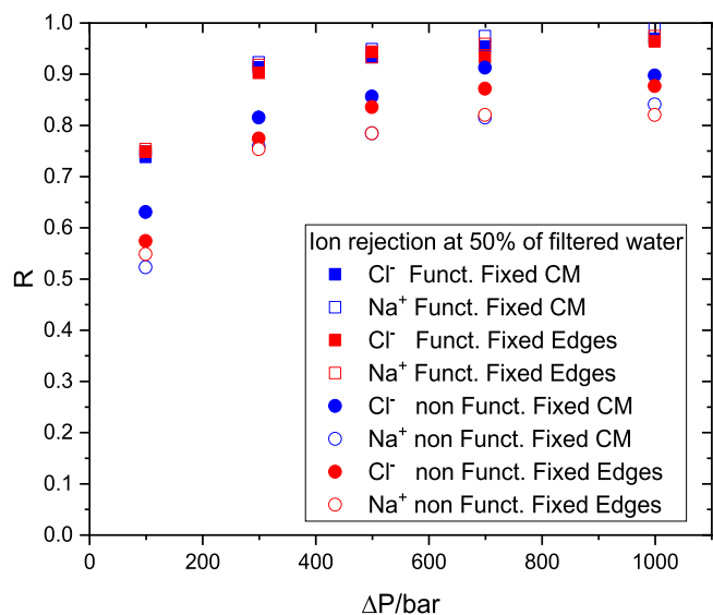
Fig. 11. The fraction of rejected ions as a function of the applied pressure difference. The y-axis error margins are below 2 %.
