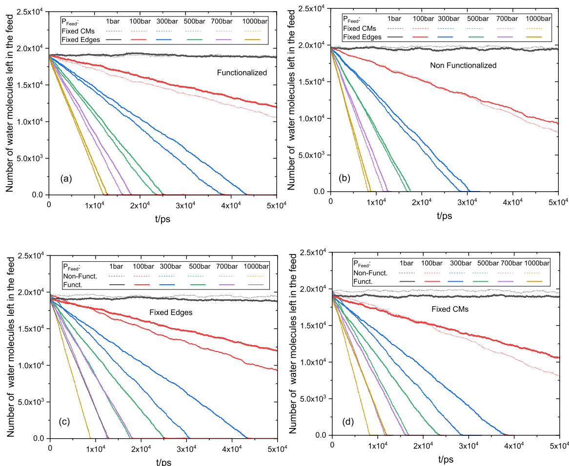
Fig. 5. Comparison of the water migration from the feed reservoir in the (a) functionalized, (b) non-functionalized, (c) fixed edges and (d) fixed CMs models.
