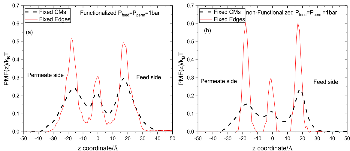
Fig. 7. PMF( z ) in units of k_B T for (a) the functionalized and (b) the non-functionalized models.
