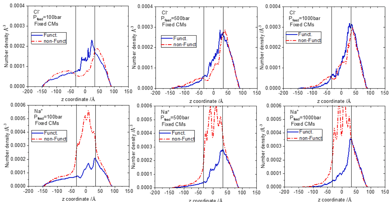
Fig. 12. z-coordinate number density profiles for the chlorine (top row) and the sodium (bottom row) ions, at different feed pressures for the fixed CMs models. Vertical lines denote the boundaries of the membrane. The feed side lies on the positive values of the z coordinate.
