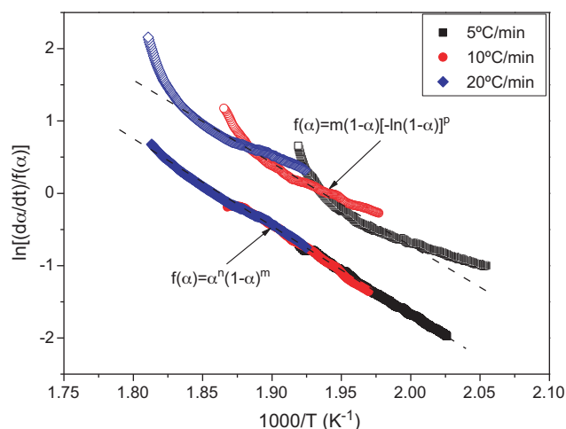
Fig. 7. Plot of \ln[(d\alpha/dt)/f(\alpha)] versus T^{-1} using two kinetic models for f(\alpha) , obtained from PHB degradation at various heating rates.
