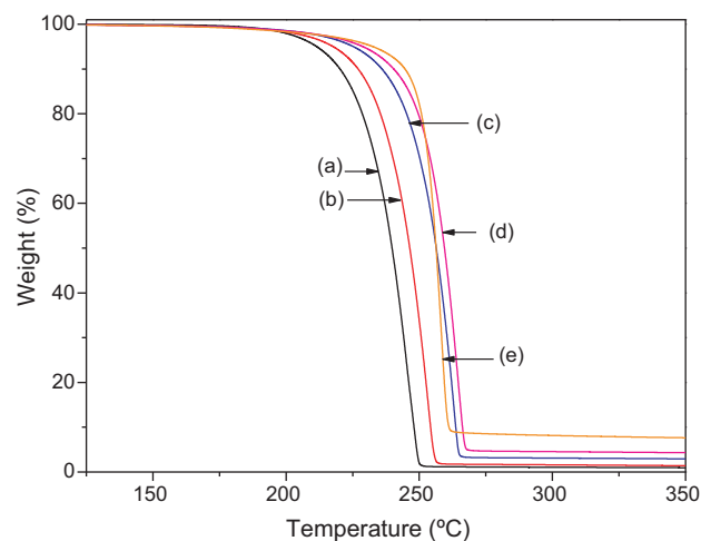
Fig. 2. Thermal degradation curves of PHB (a) and PHB nanocomposites with 1 wt% (b), 3 wt% (c), 5 wt% (d) and 10 wt% C 18 NMMT (e) after heating at 5 °C/min.
