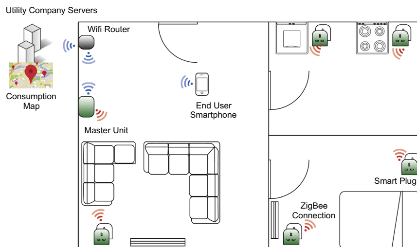
Fig. 1. Overall system architecture. Red waves indicate ZigBee connection and blue waves indicate Wifi or WAN connections. (For interpretation of the references to color in this figure caption, the reader is referred to the web version of this paper.)
