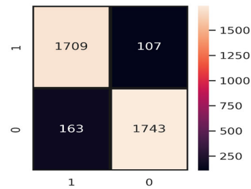
FIGURE 13. CM for SMOTE generated data using 5 fold CV.
