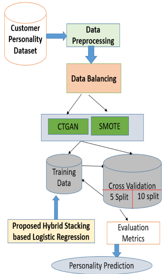
FIGURE 1. Proposed architecture for customer personality classification.
