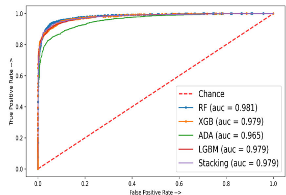
FIGURE 17. ROC for SMOTE generated data using 10-Fold CV.
