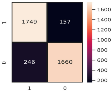
FIGURE 11. CM for 5 CV using CTGAN generated data.
