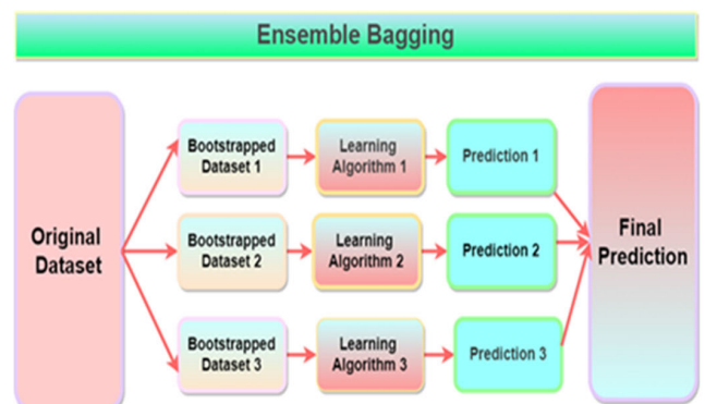
FIGURE 4. Bagging approach used for proposed system.
