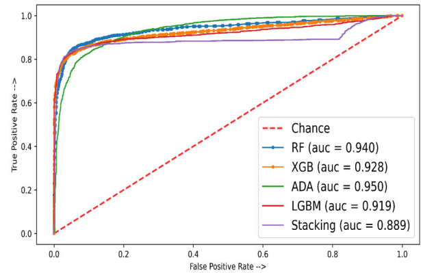
FIGURE 12. ROC using CTGAN generated data for 5 fold CV.
