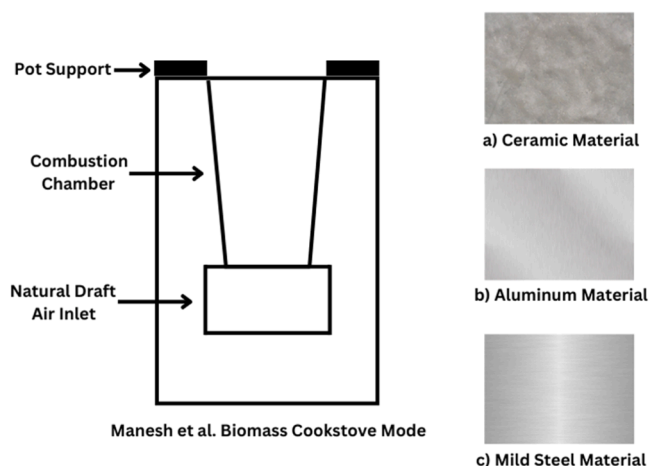
Fig. 2. Combustion chamber and relevant materials used by Mensah et al (Boafo-Mensah et al., 2020).
