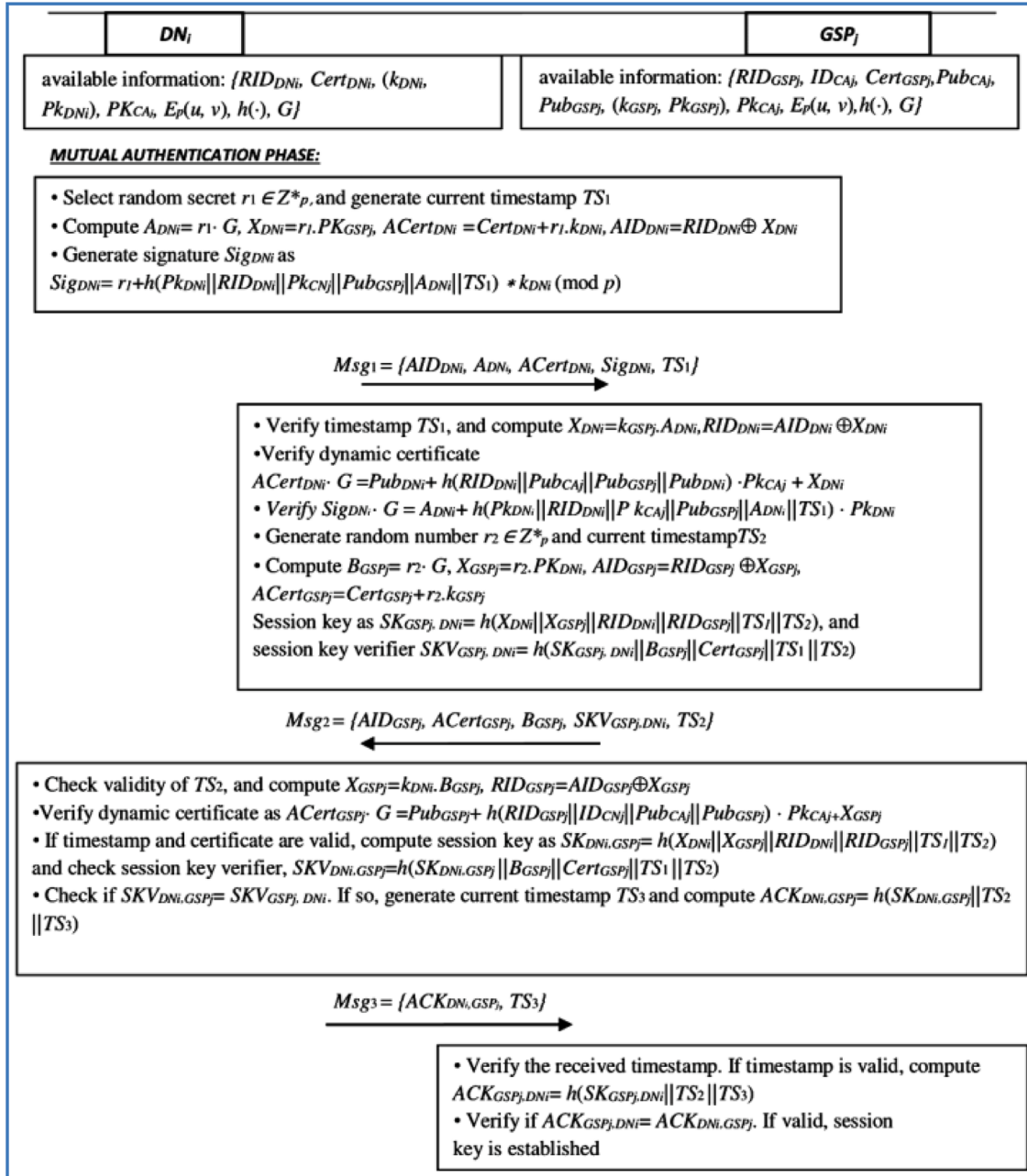
Fig. 3. Proposed mutual authentication.
