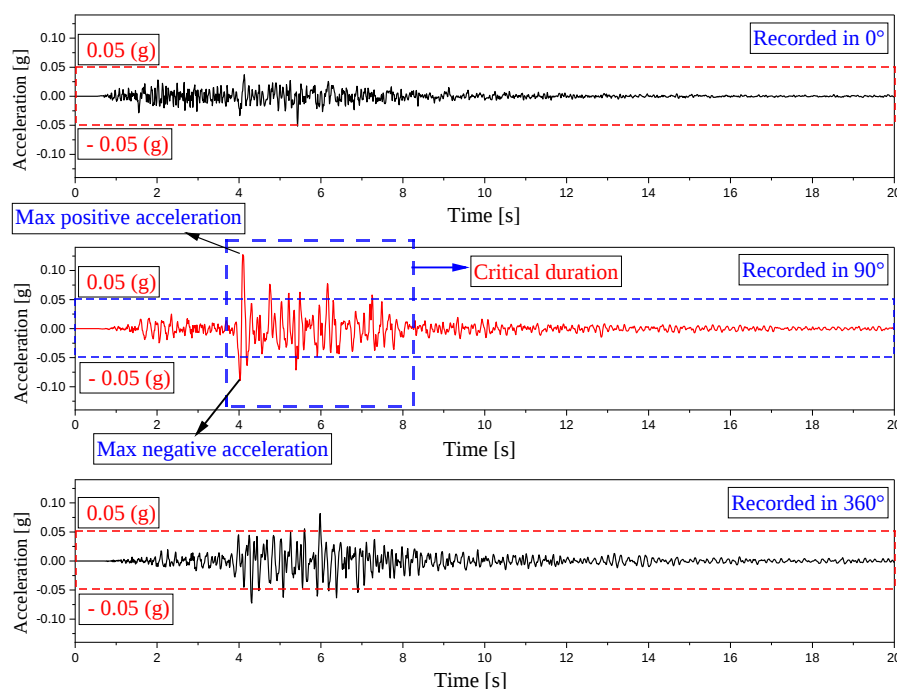
Figure 2. Ground acceleration of earthquake [31]
