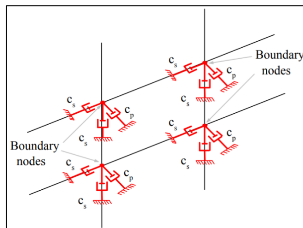
Figure 4. The boundary condition for each node [32]
