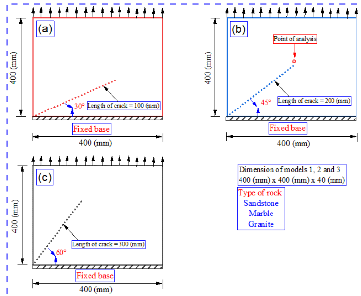
Figure 3. Simulated models 1, 2, and 3, considering types of rocks
