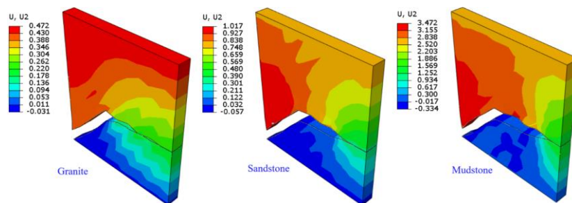
Figure 8. Displacement in the vertical direction of all models in the final stage of crack propagation with a preexisting fracture angle of 45^\circ for granite, sandstone, and mudstone
