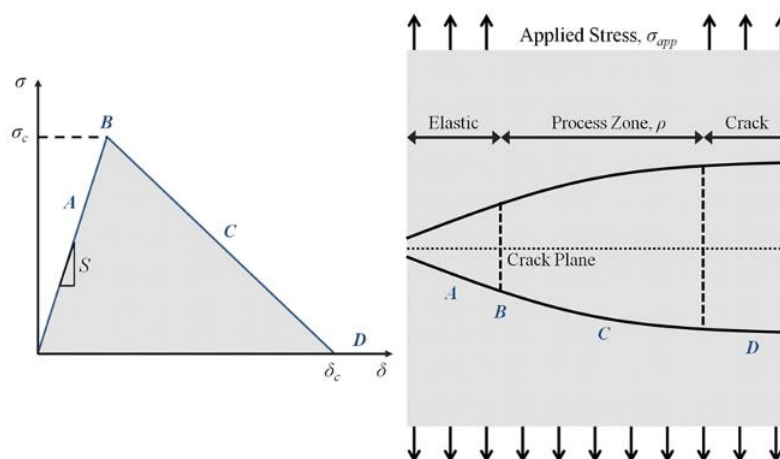
Figure 5. Graphical representation to explain the cohesive zone of the simulated model with the crack traction-separation constitutive performance [35]
