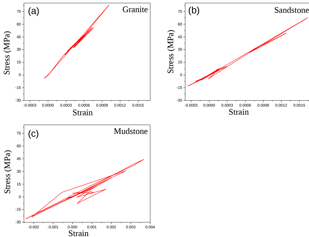
Figure 9. Stress-strain for granite, sandstone, and mudstone
