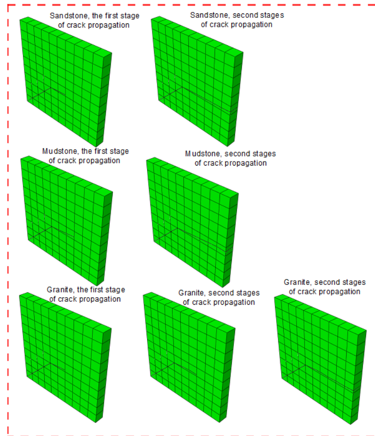
Figure 7. The preexisting fracture angle at 45^\circ and propagation of the fracture in sandstone, mudstone, and granite
