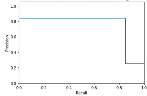
Average precision score [Decision Tree Classifier Model], micro-averaged over all classes: AP=0.75
