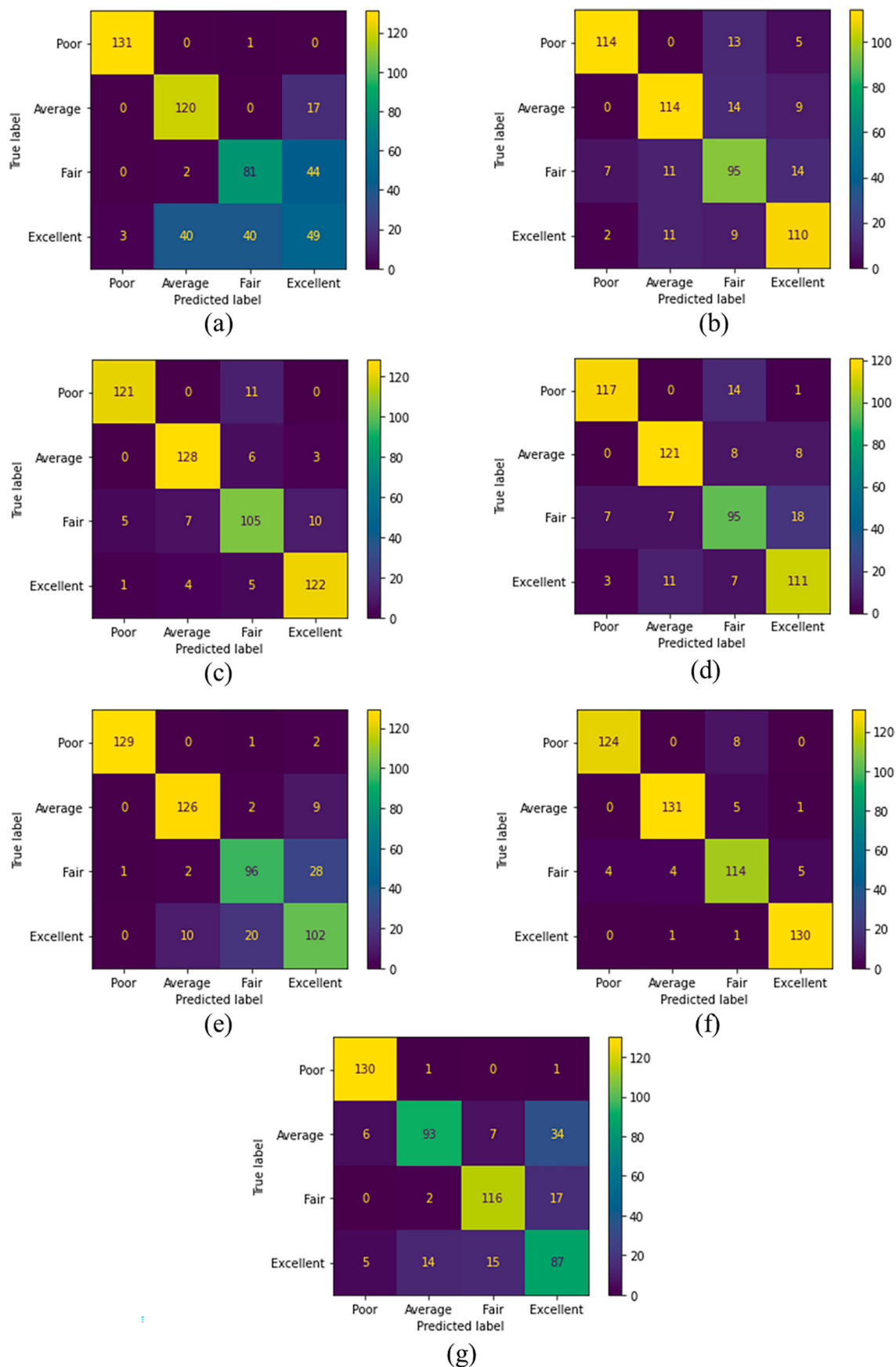
Fig. 4. Confusion matrix (Imputation with median and standard scaler) a) Logistic regression, b) Decision tree classifier c) Random Forest classifier d) XGB classifier e) MLP classifier f) CATBoost classifier g) SVM classifier.
