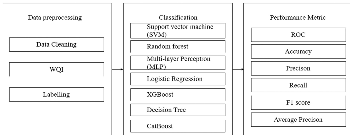
Fig. 1. Methodology of the proposed system.
