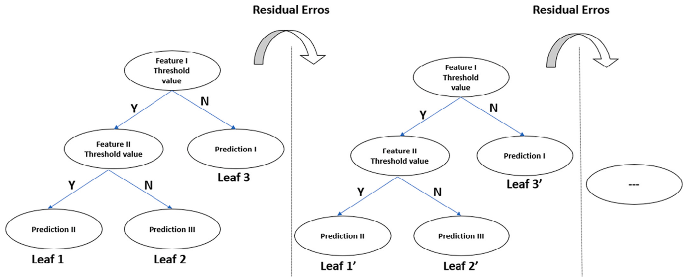
Fig. 3. Schematic diagram of XGBoost trees.
