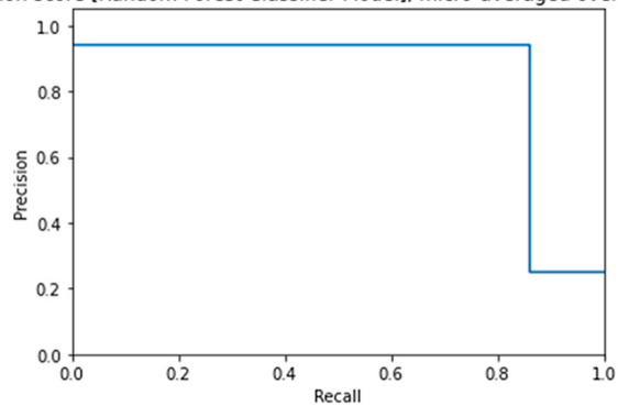
Average precision score [Random Forest Classifier Model], micro-averaged over all classes: AP=0.84
