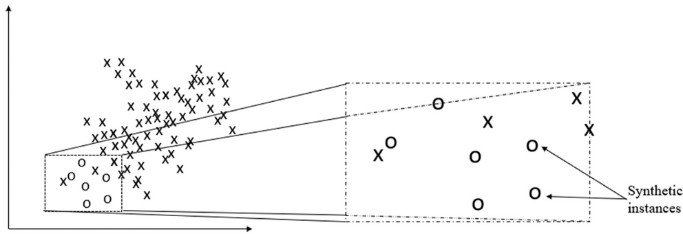
Fig. 2. Schematic diagram of the synthetic instances of the SMOTE algorithm.
