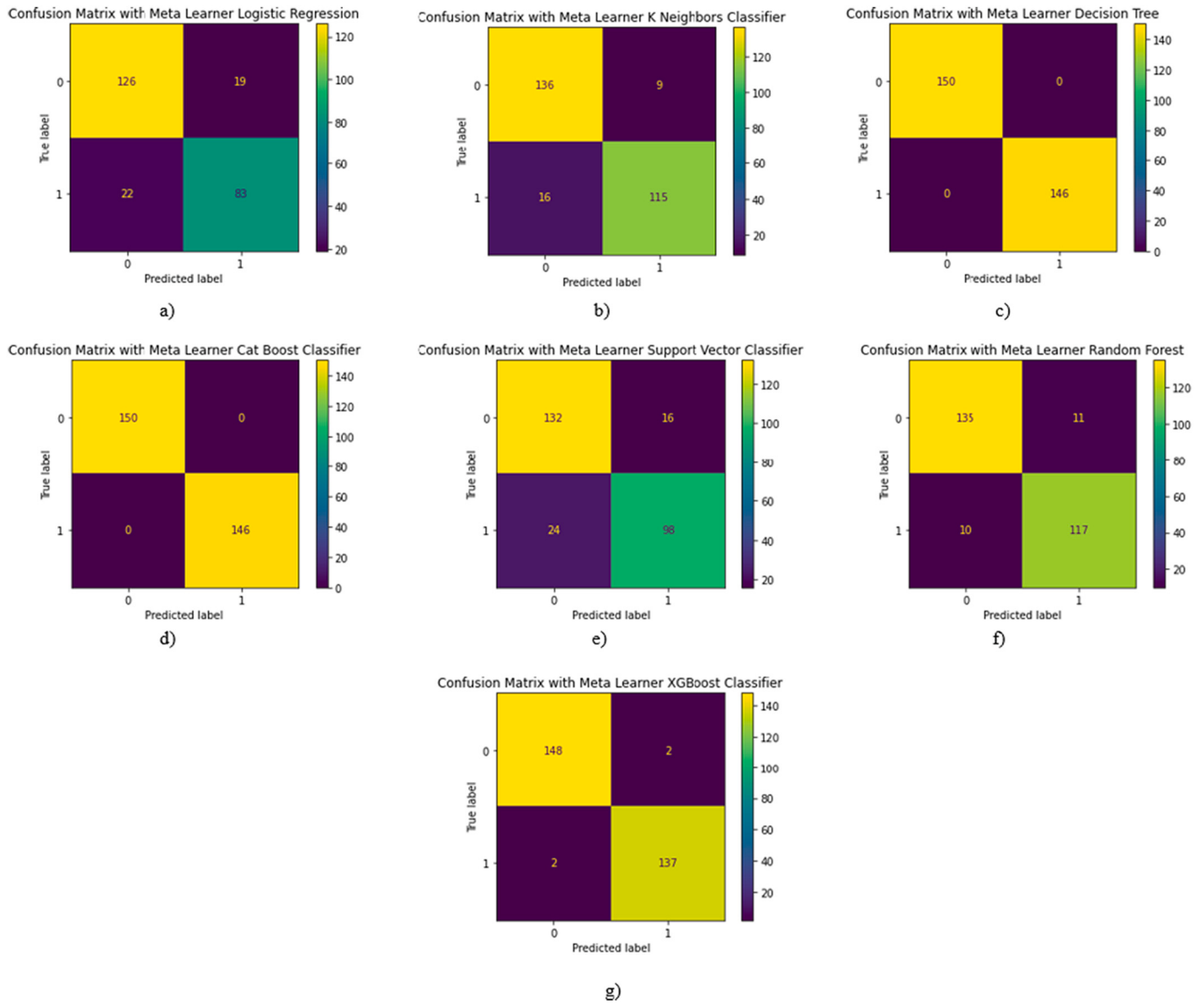
Fig. 9. Meta learner-confusion matrix: a) Logistic regression, b) KNN classifier, c) Decision tree classifier, d) CATBoost classifier, e) SVM classifier, f) Random Forest classifier, and, g) XGB classifier.
