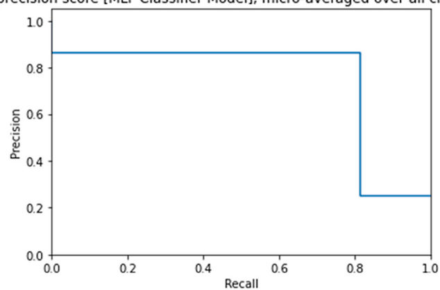
Average precision score [MLP Classifier Model], micro-averaged over all classes: AP=0.75
