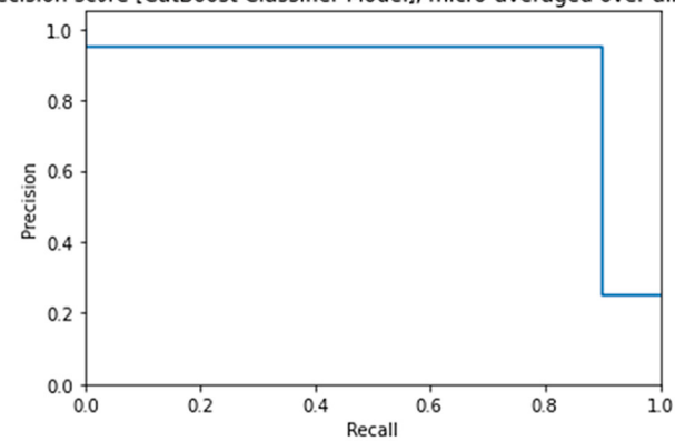
Average precision score [CatBoost Classifier Model], micro-averaged over all classes: AP=0.88
