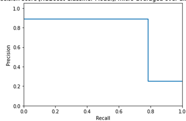
Average precision score [XGBoost Classifier Model], micro-averaged over all classes: AP=0.75
