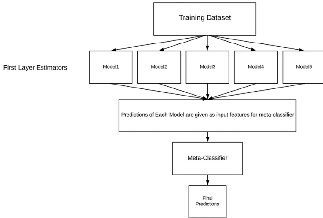
Fig. 8. The architecture of a Stacked Model.
