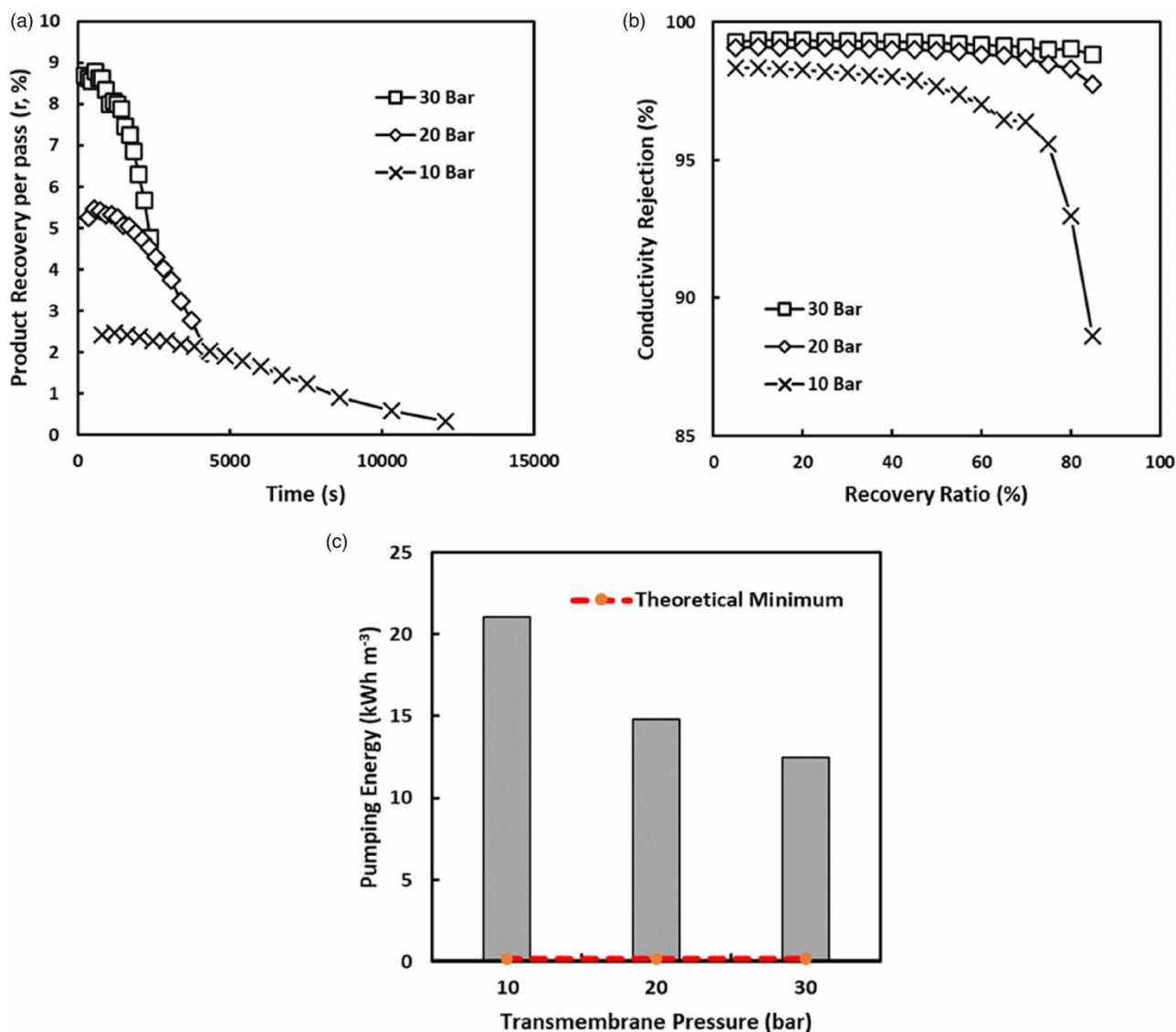
Figure 3 | Effect of TMP on (a) RR per pass; (b) rejection; and (c) pumping energy for a single 1812 element. Experimental conditions: CFV 0.084 m s -1 ; 25 °C; feed volume 10 L; RR >85%; and feed concentration 0.056 M NaCl (equivalent conductivity to blackwater).
