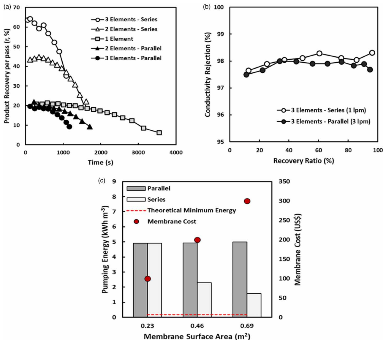
Figure 5 | Investigating a stage design for the batch open-loop RO at fixed velocity, increasing the total membrane area through increasing module number in series or in parallel: (a) impact on product recovery per pass; (b) rejection; (c) pumping energy and membrane cost. Experimental conditions: CFV 0.028 \text{ m s}^{-1} ; 25^\circ \text{C} ; feed volume 10 L; concentration 0.056 M NaCl; and TMP 30 bar.
