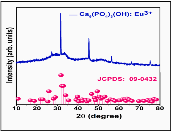
Fig. 2. XRD spectrum of Han: Eu 3+ NCs.
