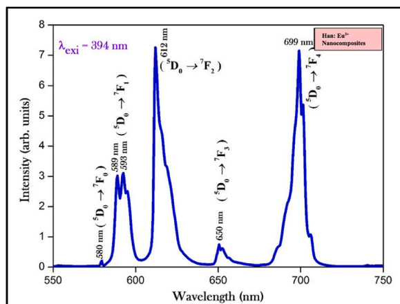
Fig. 8. Emission Spectrum of Han: Eu 3+ NCs.
