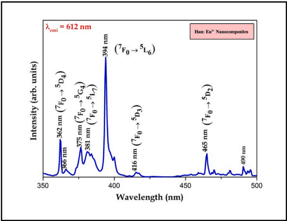
Fig. 7. The excitation spectrum of Han: Eu 3+ NCs.
