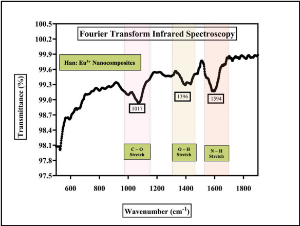
Fig. 1. FTIR spectrum of Han: Eu 3+ nanocomposites.
