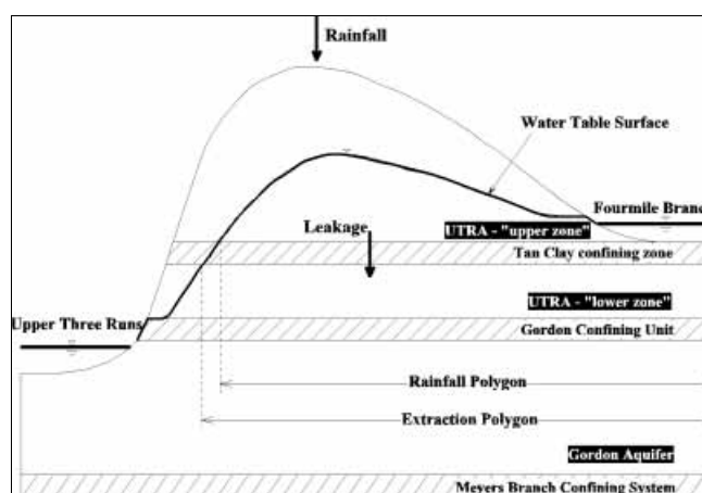
Figure 2 | Idealized cross-section of the GSA aquifer system (modified after Flach and Harris 1999).
