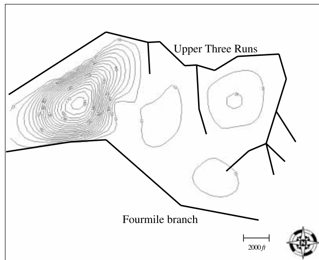
Figure 7 | Variance of the mean hydraulic head distribution.
