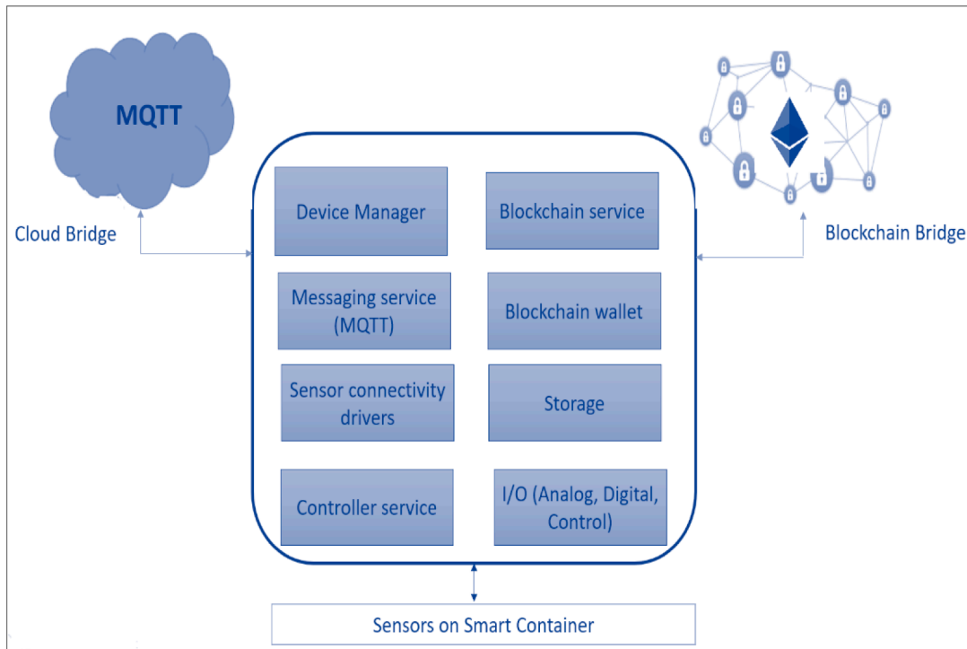
Fig. 5. MQTT server for blockchain-based food safety use case. (Majdalawieh et al., 2021).
