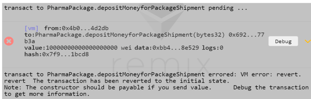
Fig. 15. Logs showing error: when consumer deposits amount before package-check function 1 . ( 1 Code available at: https://github.com/nisharan/OnlineSupplyChainManagement ).
