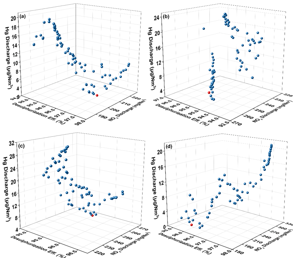
Fig. 7. The optimal solution estimated by NSGA-II under different operating values taken from the operating range of inlet dust, inlet SO 2 , and inlet NO x as a) minimum, b) middle, c) maximum, and d) full operating range. The optimal solution is selected by TOPSIS and is shown by red spot.
