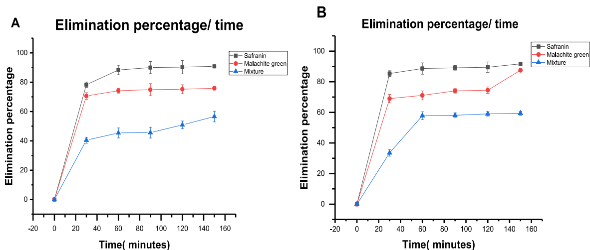
Fig. 7. Effect of temperature on the removal of dyes (A) 35 °C (B) 50 °C qt versus time graph has shown a similar pattern that high adsorption happens within the first 30 min and then the slope becomes linear.
