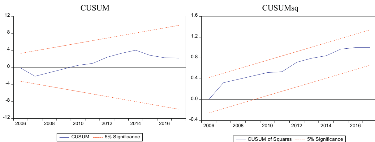
Fig. 2. Plot of the cumulative sum and cumulative sum of the squares of recursive residuals.
