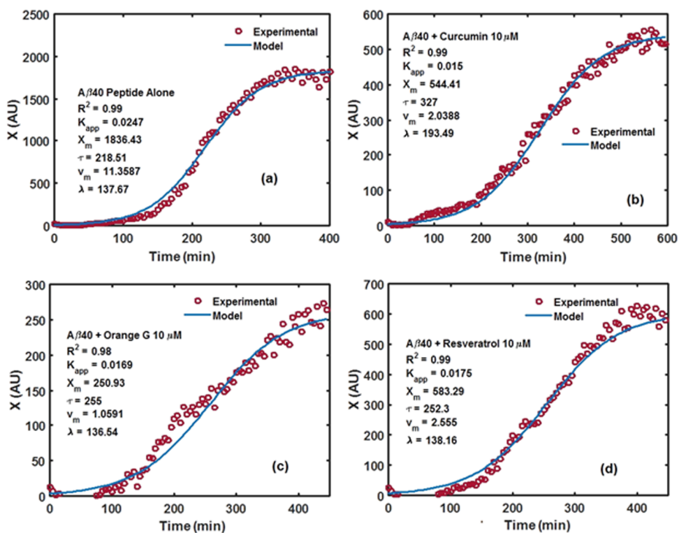
Figure 4. Comparison of fluorescence intensity ( X ) and time obtained from the fitted model and the experimental data for (a) A \beta 40 alone, (b) A \beta 40 and curcumin at 10 \mu\text{M} , (c) A \beta 40 and orange G at 10 \mu\text{M} , and (d) A \beta 40 and resveratrol at 10 \mu\text{M} .
