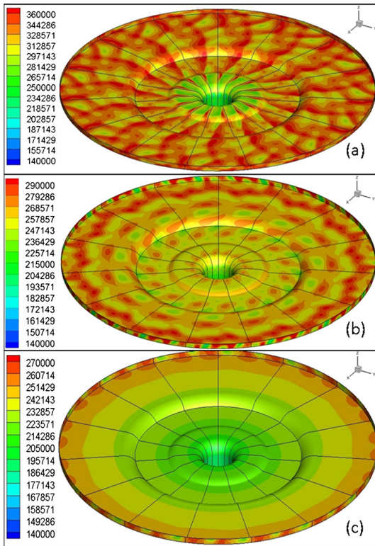
Fig. 15. Instantaneous static pressure in Pa on the impeller back plate at: (a) surge, (b) design, (c) near choke.
