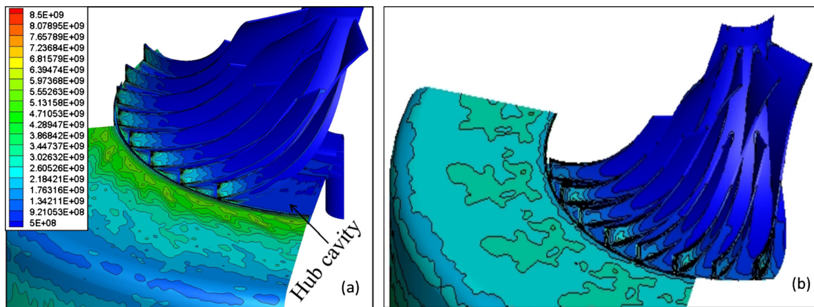
Fig. 24. Surface dpdt RMS on compressor stage walls for: (a) with cavity, (b) without cavity.
