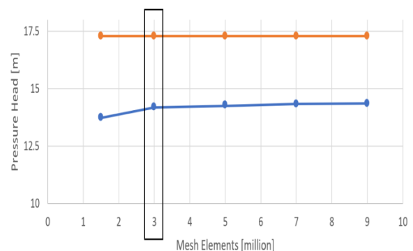
Fig.5: Mesh Independency Test
