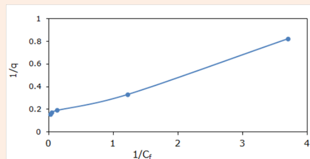
Figure 7: Langmuir Isotherm for Cadmium (Cd ++ ).
