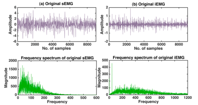
Fig. 3. (a) Original sEMG signal with its frequency spectrum, and (b) Original iEMG signal with its frequency spectrum.
