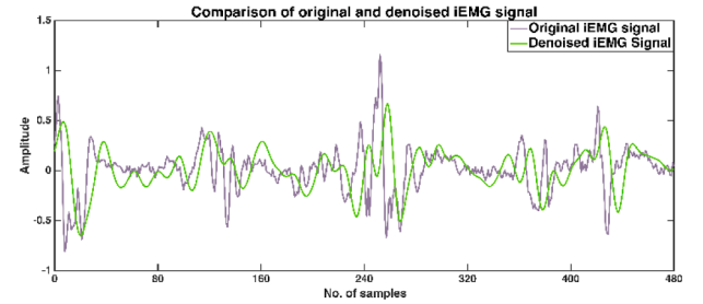
Fig. 14. Comparison between the original and denoised signal for iEMG.
