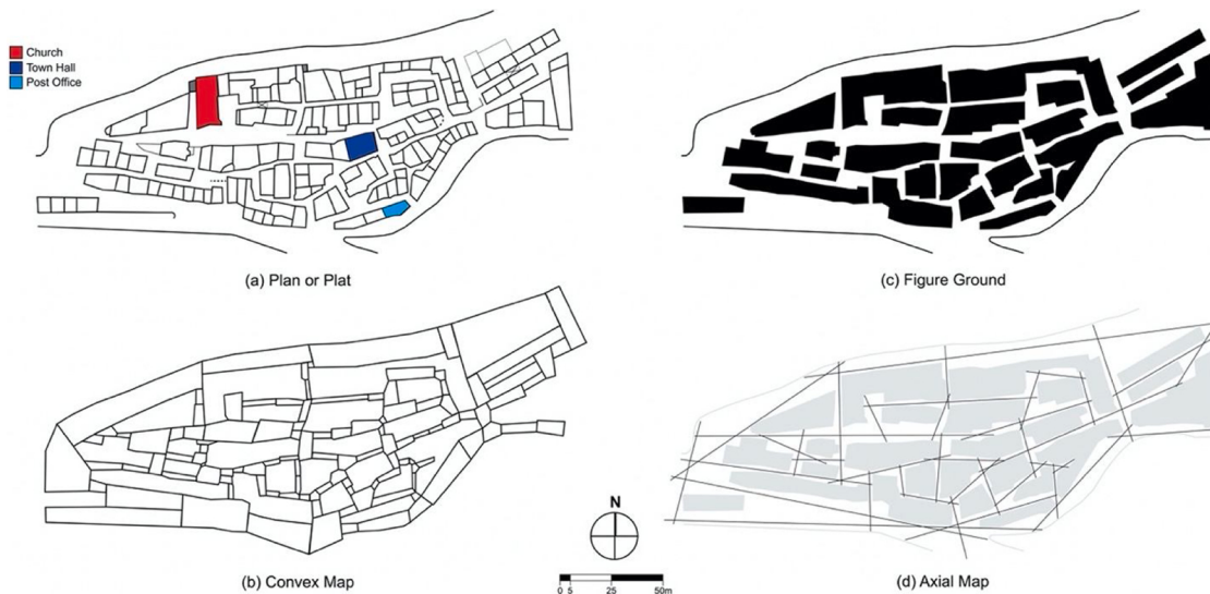
Fig. A3. The procedure for modeling settlements based on the (a) plan/plot, (b) convex map, (c) figure-ground, and (d) axial map for the layout of Gassin in the Var region of France circa 1980 (Images: Mark David Major after Hillier and Hanson, 1984).
