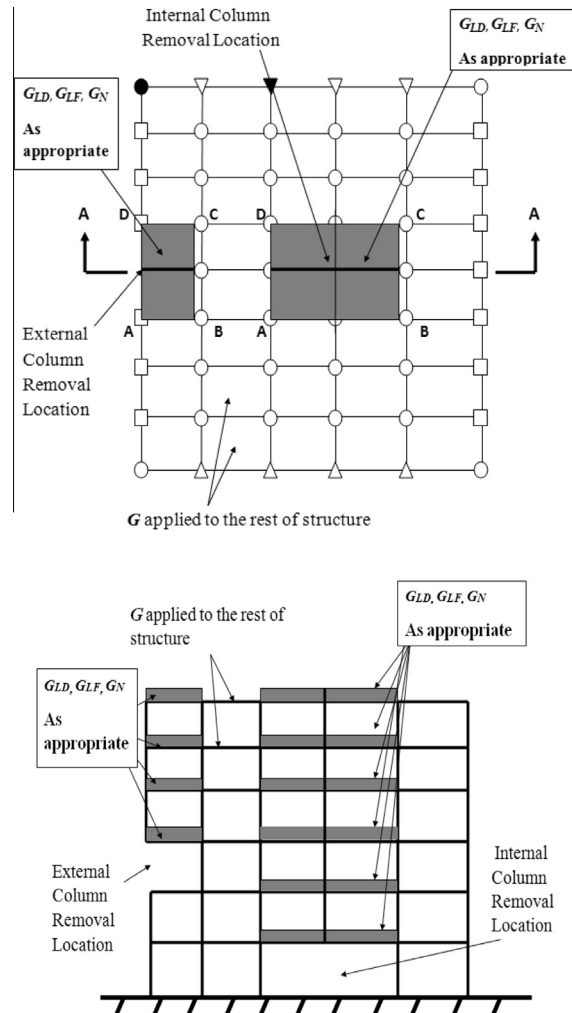
Fig. 2. Gravity load combinations on bays adjacent to the removed column and bays away from the removed column.
