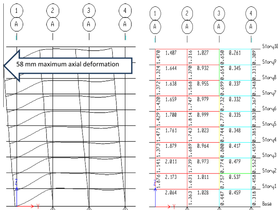
Fig. 6. (a) Deformed shape due to progressive collapse loading. (b) Demand/capacity ratio due to progressive collapse load combination.
