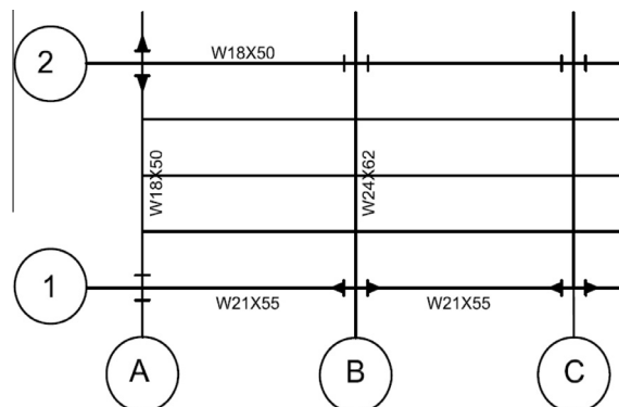
Fig. 5. Partial plan view at location where corner column A1 will be notionally removed at the base level.
