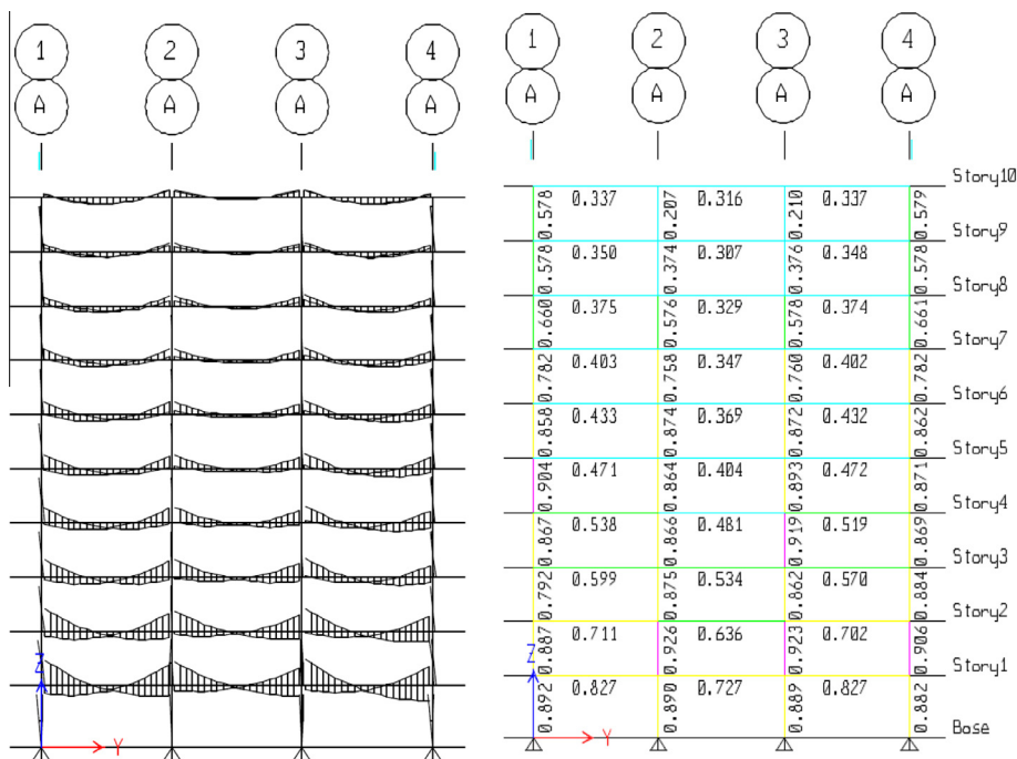
Fig. 4. (a) Bending moment diagram (b) demand/capacity ratio.
