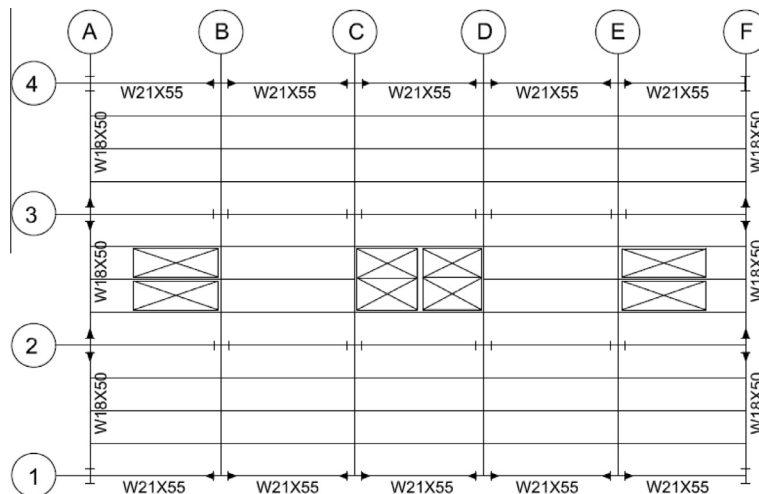
Fig. 3. First floor plan of 10-story steel framed building with perimeter moment frame and Improved WUF moment connections.
