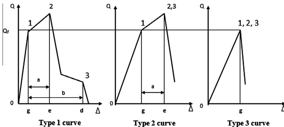
Fig. 1. Force-deformation curves for classification of actions as tension-controlled or force-controlled.
