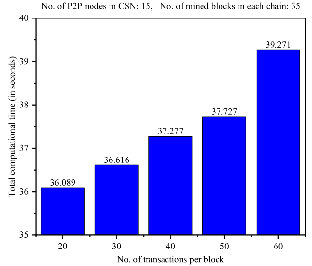
Fig. 7. Blockchain simulation results for Case 2.
