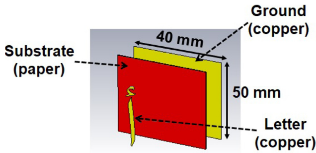
Fig. 2. Structure and dimensions of designed Arabic letter tags (example of letter (Alf)).
