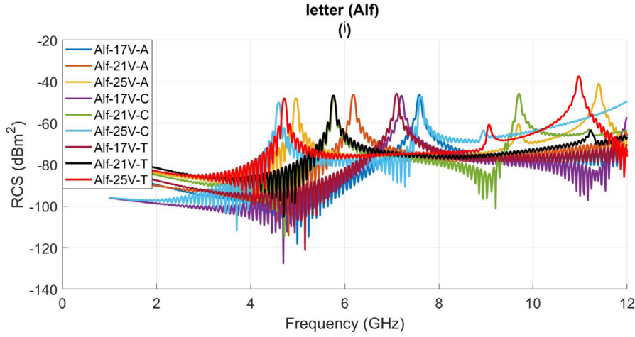
Fig. 11. Cross polar RCS Results of letter tag Alf (ا) for Arial, Calibri, and Times New Roman font types of sizes 17 mm, 21 mm, and 25 mm.
