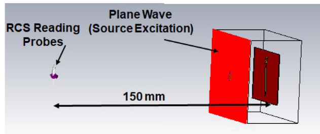
Fig. 3. Full-wave numerical analysis setup for realized Arabic letter tags.
