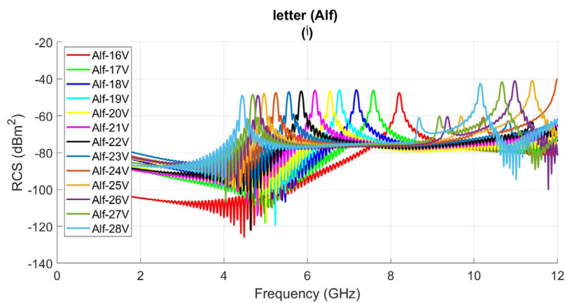
Fig. 6. Cross polar RCS results of letter tag Alf (ا) for Arial font type in different sizes.
