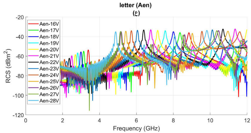
Fig. 8. Cross polar RCS Results of letter tag Aen (ع) for Arial font type in different sizes.
