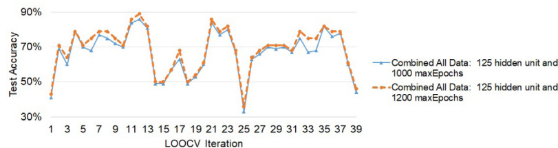
Fig. 23. Comparison of test accuracies when utilizing LOOCV with different network settings for combined dataset.
