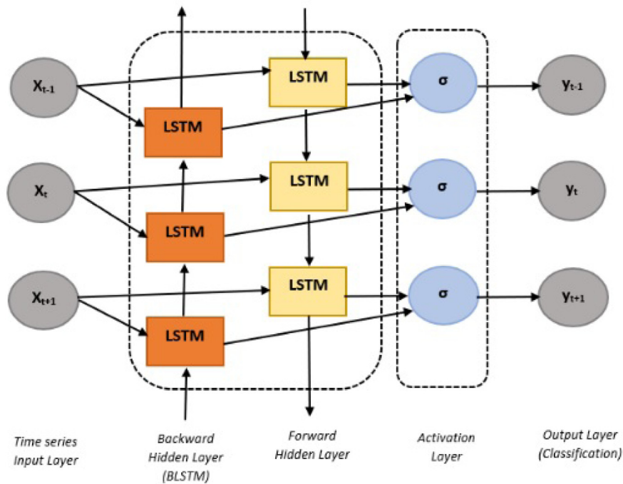
Fig. 18. Architecture of a simple BiLSTM network.
