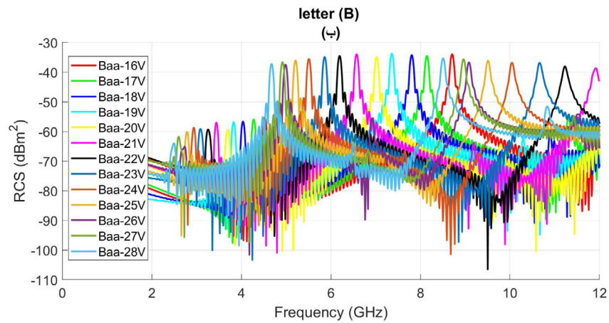
Fig. 9. Cross polar RCS Results of letter tag Baa (ب) for Arial font type in different sizes.
