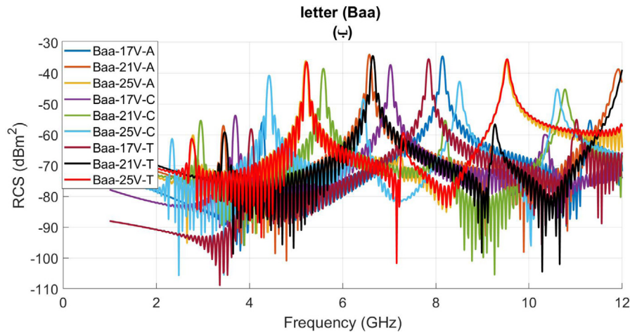
Fig. 13. Cross polar RCS Results of letter tag Baa (بَا) for Arial, Calibri, and Times New Roman font type of sizes 17 mm, 21 mm, and 25 mm.
