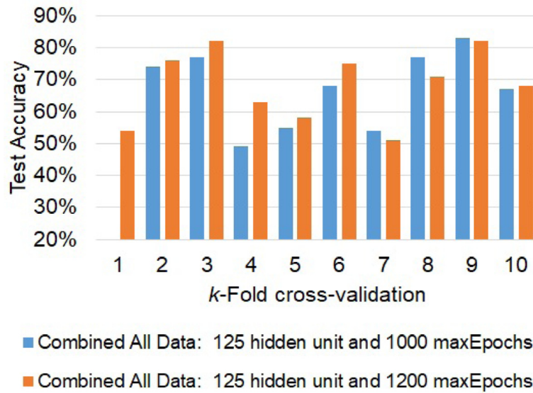
Fig. 21. Comparison of test accuracies when utilizing k -fold cross-validation with different network settings for combined all font types and sizes data.
