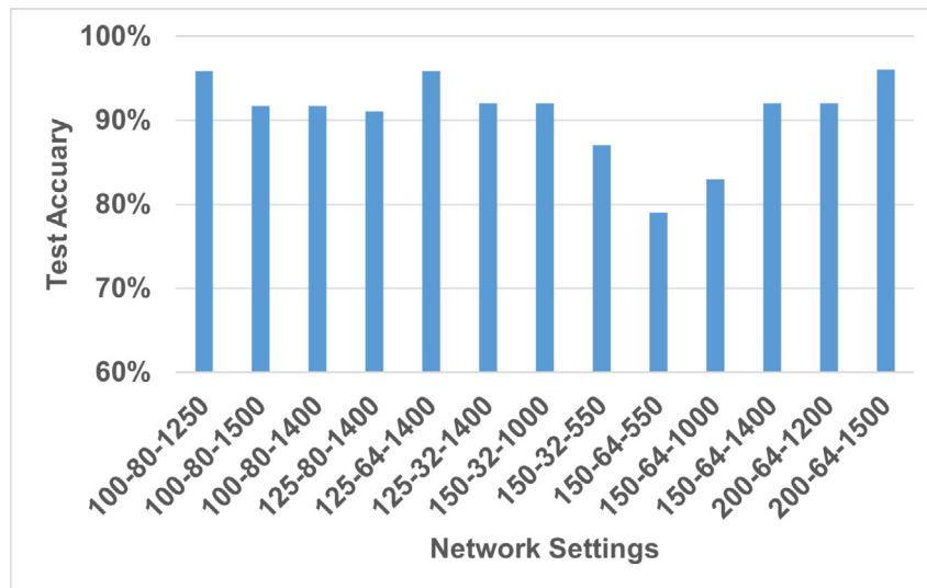
Fig. 25. Test accuracy results of tag detection after removing four tags (ب, ج, ظ, و) from the data set in different hyper-parameters setting.
