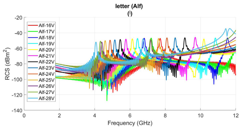
Fig. 7. Cross polar RCS results of letter tag Alf (ا) for Calibri font type in different sizes.
