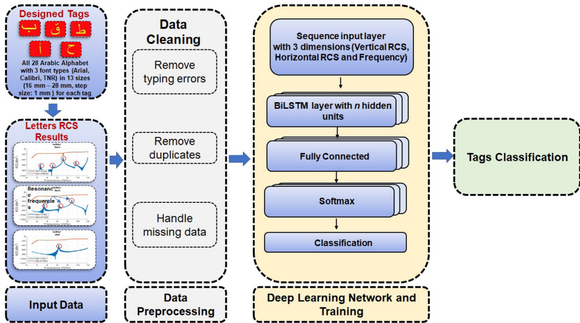
Fig. 16. Proposed deep learning-based system framework for the robust detection and classification of chipless Arabic letters (the n represents hidden unit of BiLSTM network with tested values of 100/125/150 for this study).
