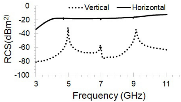
Fig. 1. Typical RCS electromagnetic signature of a chipless Arabic letter tag.
