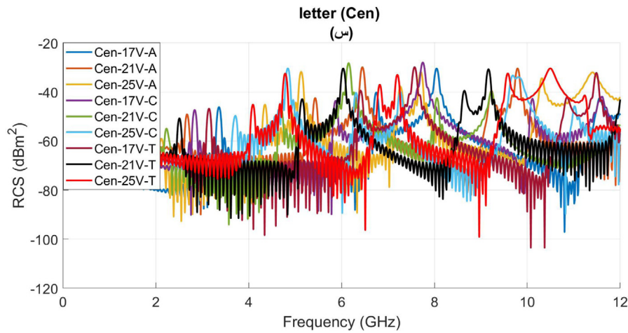
Fig. 14. Cross polar RCS Results of letter Cen (سِن) for Arial, Calibri, and Times New Roman font types of sizes 17 mm, 21 mm, and 25 mm.
