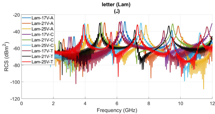
Fig. 15. Cross polar RCS Results of letter Lam (لَم) for Arial, Calibri, and Times New Roman font types of sizes 17 mm, 21 mm, and 25 mm.
