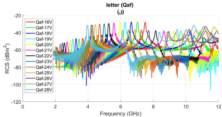
Fig. 10. Cross polar RCS results of letter tag Qaf (ق) for Times New Roman font type in different font sizes.
