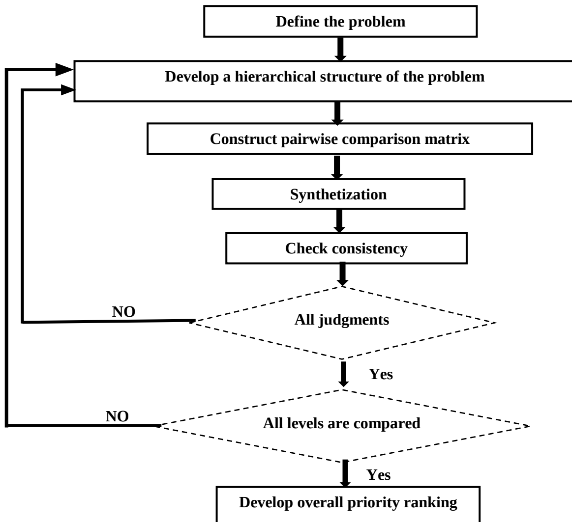
Figure 5: Flow Diagram of AHP Method Employed
