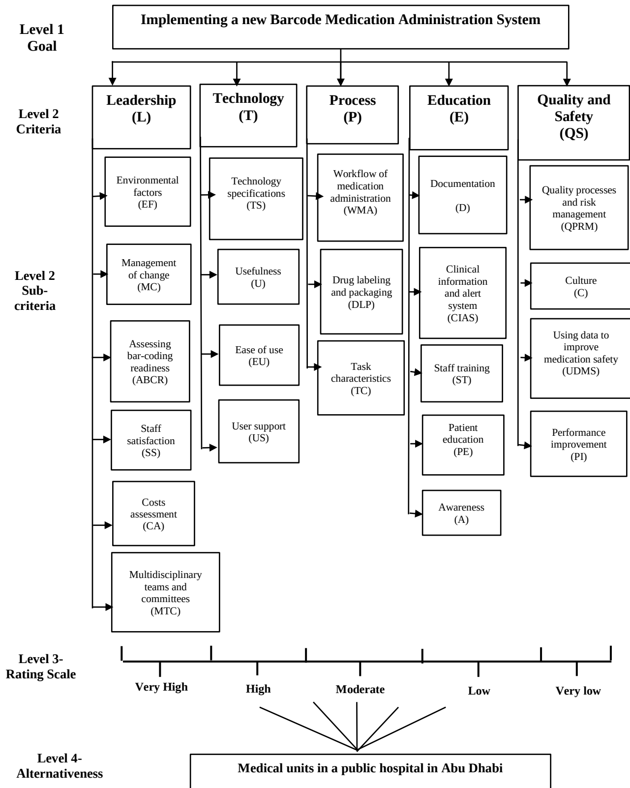
Figure 4: AHP Model for Evaluating the Implementation of BCMA System
